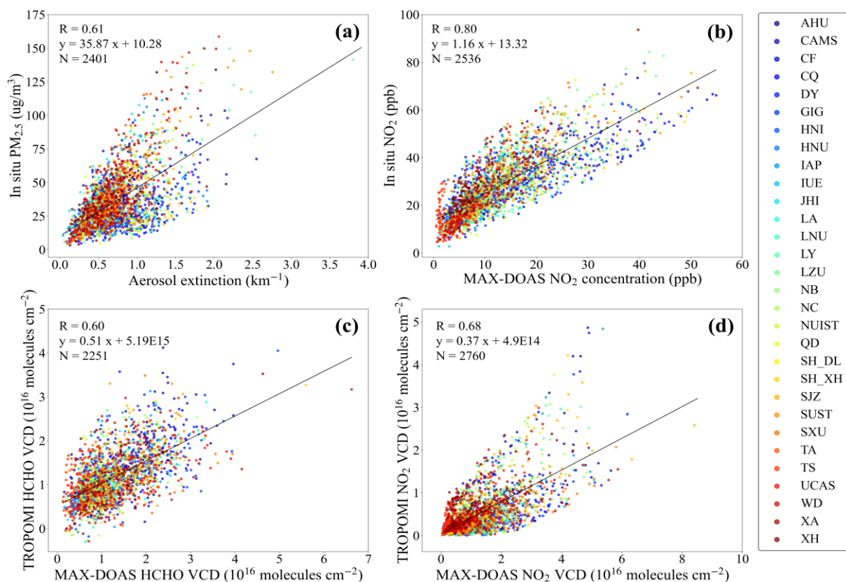
Figure 10. Correlation analysis (a) of PM 2.5 measured by CNECM and surface AEC (0–100 m) measured by MAX-DOAS, (b) of NO 2 concentration measured by CNECM and MAX-DOAS, (c) of the tropospheric HCHO VCD measured by TROPOMI and MAX-DOAS and (d) of the tropospheric NO 2 VCD measured by TROPOMI and MAX-DOAS.
