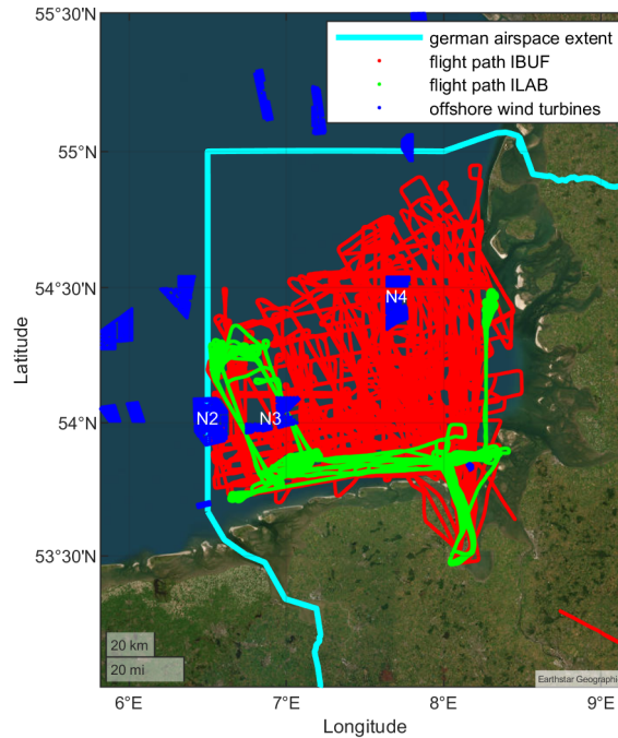
Figure 3. Overview of the airborne measurements conducted in the framework of the project X-Wakes. The light blue line indicates the borders of the German airspace for which the flight permission was valid. Wind turbines in operation on the last flight day, 11 September 2021, are displayed in dark blue. All the flight tracks of the Dornier 128 are shown in red, and the flight tracks of the Cessna F406 in green. The names of the wind park clusters N2, N3 and N4 are indicated in white letters,
