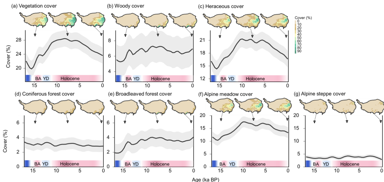
230 Figure 4: Changes in vegetation cover on the Tibetan plateau since 16 Ka BP (a-g). The solid lines represent the smoothed changes in vegetation cover using a cubic smoothing spline. The shading indicates the 95% confidence interval. Shown at the top are spatial distributions of vegetation cover at 15.2 Ka BP, 7.6 Ka BP, and 0 Ka BP.
