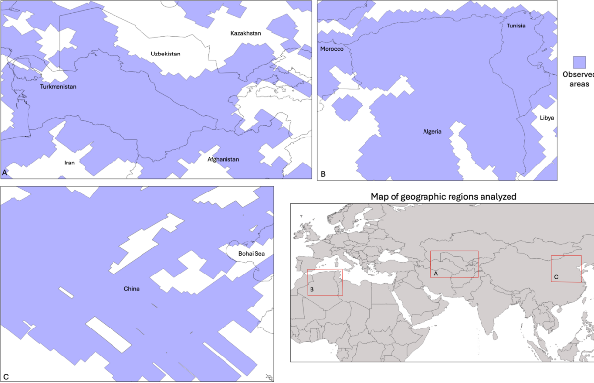
Figure S2: Map of the geographic regions where Carbon Mapper has processed data to look for super-emitting events in Turkmenistan/Uzbekistan (A; top left), Algeria (B; top right), and northeast China (C; bottom left). The bottom right plot shows a zoomed-out map view of the three regions.
