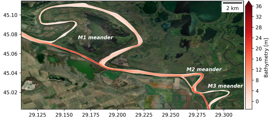
Figure 5. Map of the interpolated bathymetry in a section of the Sfantu Gheorghe branch. M1 and M3 meanders present a shallower bathymetry than their respective artificial canal, while M2 meander is deeper than its man-made cut-off channel. The background image is the Esri World Imagery basemap (ESRI, 2025)
