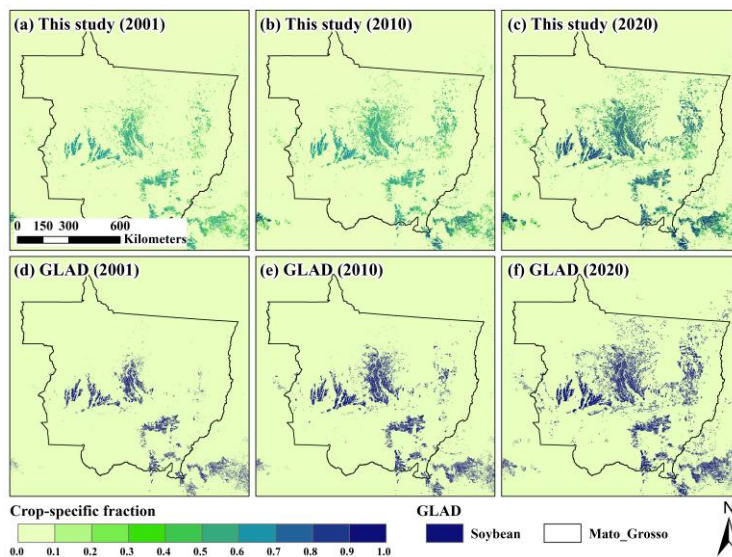
Figure 12. Temporal visual comparison of soybean fraction with GLAD.
