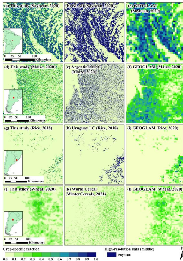
690 Figure 11. Visual comparison of crop-specific maps between this study and other datasets. The left column shows the crop-specific maps in this study, with high-resolution data in the middle and coarse-resolution data on the right. Panels b, e, h, and l were also used as input layers in generating the 2020 base map.
