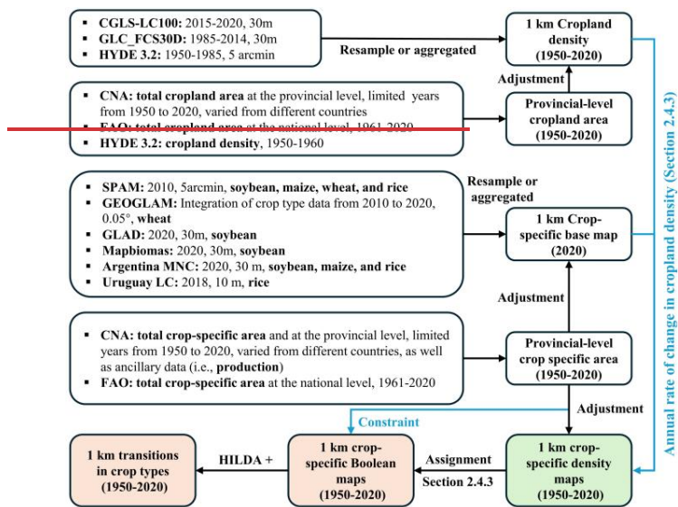
Figure 2. The flow chart in this study. CNA refers to Census National Agriculture.
