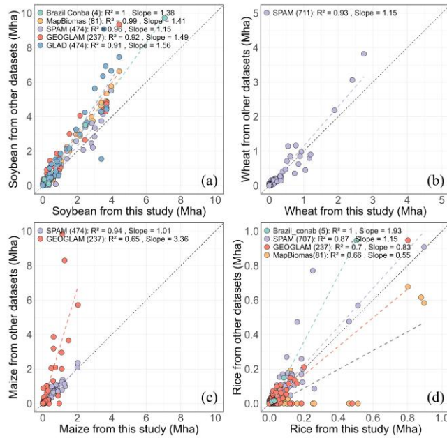
560 Figure 6. Comparison of crop type areas between this study and existing datasets ( gridded datasets that were not involved in reconstruction process , i.e., Argentina MNC , Brazil Conba (2017-2020) , MapBiomass , (2000, 2005, 2010) , SPAM , (2000, 2005) , GEOGLAM , (2020) , GLAD , WorldCereal , and Uruguay LC (2005, 2010) ) at the provincial level. (a) Soybean; (b) Wheat; (c) Maize; (d) Rice. The numbers in parentheses represent the total number of samples.
