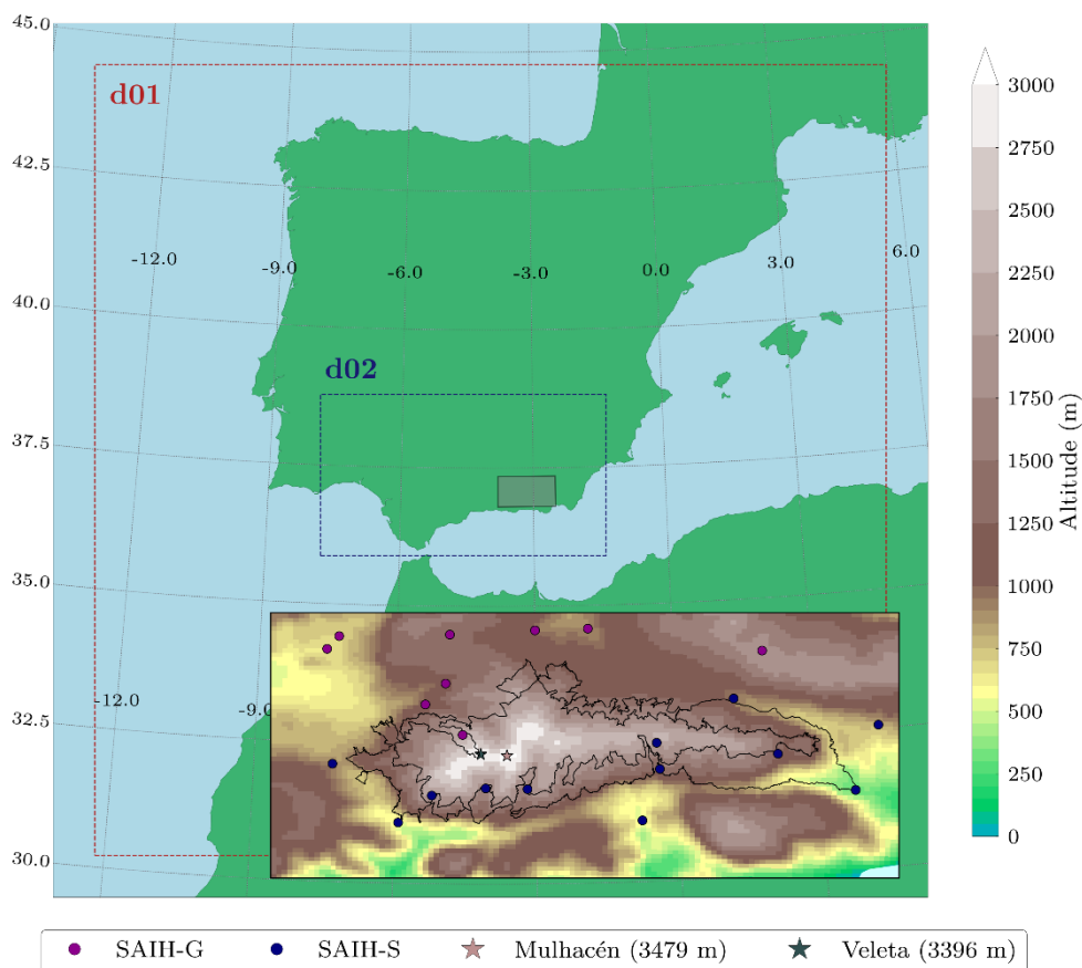
90 Figure 1: WRF model configuration with two one-way domains: the parent domain (d01), which covers the Iberian Peninsula (IP) with 5 km spatial resolution, and the inner domain (d02), which spans the Andalusia region with 1 km spatial resolution. The area covered by HighResClimNevada is depicted in the inner figure at the bottom right, including the boundaries of both the Natural and National Parks of Sierra Nevada (black contours). The shading colors in this subfigure denote the elevation stated in meters above mean sea level, while the dots represent the locations of stations from the HidroSur automatic Hydrological Information System (SAIH-S) and the Guadalquivir automatic Hydrological Information System (SAIH-G). 95
