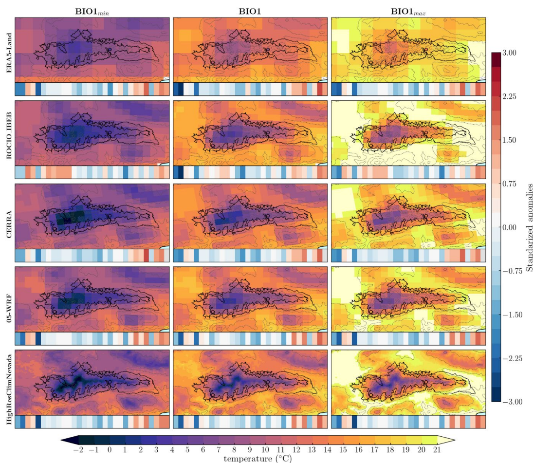
390 Figure 3: Annual mean of the daily minimum, mean, and maximum temperatures ( BIO1_{min} , BIO1 , and BIO1_{max} ) for each reference dataset (ERA5-Land, ROCIO_IBEB, and CERRA) as well as for downscaled data (05-WRF and HighResClimNevada). The dots in each panel represent the temperature recorded by SAIH stations, and the black solid lines display the National and Natural Park boundaries. Normalized anomalies for SN Natural Park over the period 2001-2020 for each database are shown below the corresponding spatial map in the form of warming stripes. In this representation, red colors indicate positive standardized anomalies and blue colours negative values compared to the mean value for the whole period.
