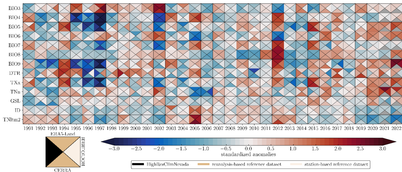
500 Figure 6: Normalized temperature anomalies for bioclimatic variables and ETCCDI extreme indices. Anomalies are calculated using the mean and standard deviation in a common period (1991-2022) of each database and spatially averaged across the SN Natural Park. Black triangles indicate that there is no value for that year in the specified database. The legend depicts the sequence of the data in each square (in black, HighResClimNevada), with the nature of each database marked by color.
