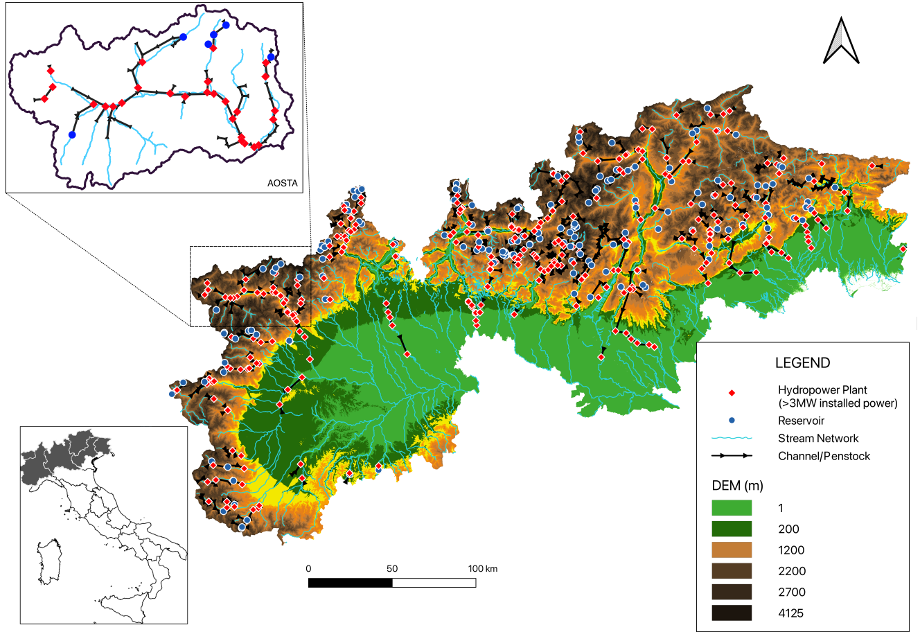
Figure 1. Distribution map of hydropower plants identified in the IAR-HP database, including relevant reservoirs for storage-based plants and diversion channels linking these systems. The top-left inset shows the Aosta province, highlighting the level of detail captured in IAR-HP. The bottom-left inset shows the covered area of IAR-HP in Italy.
