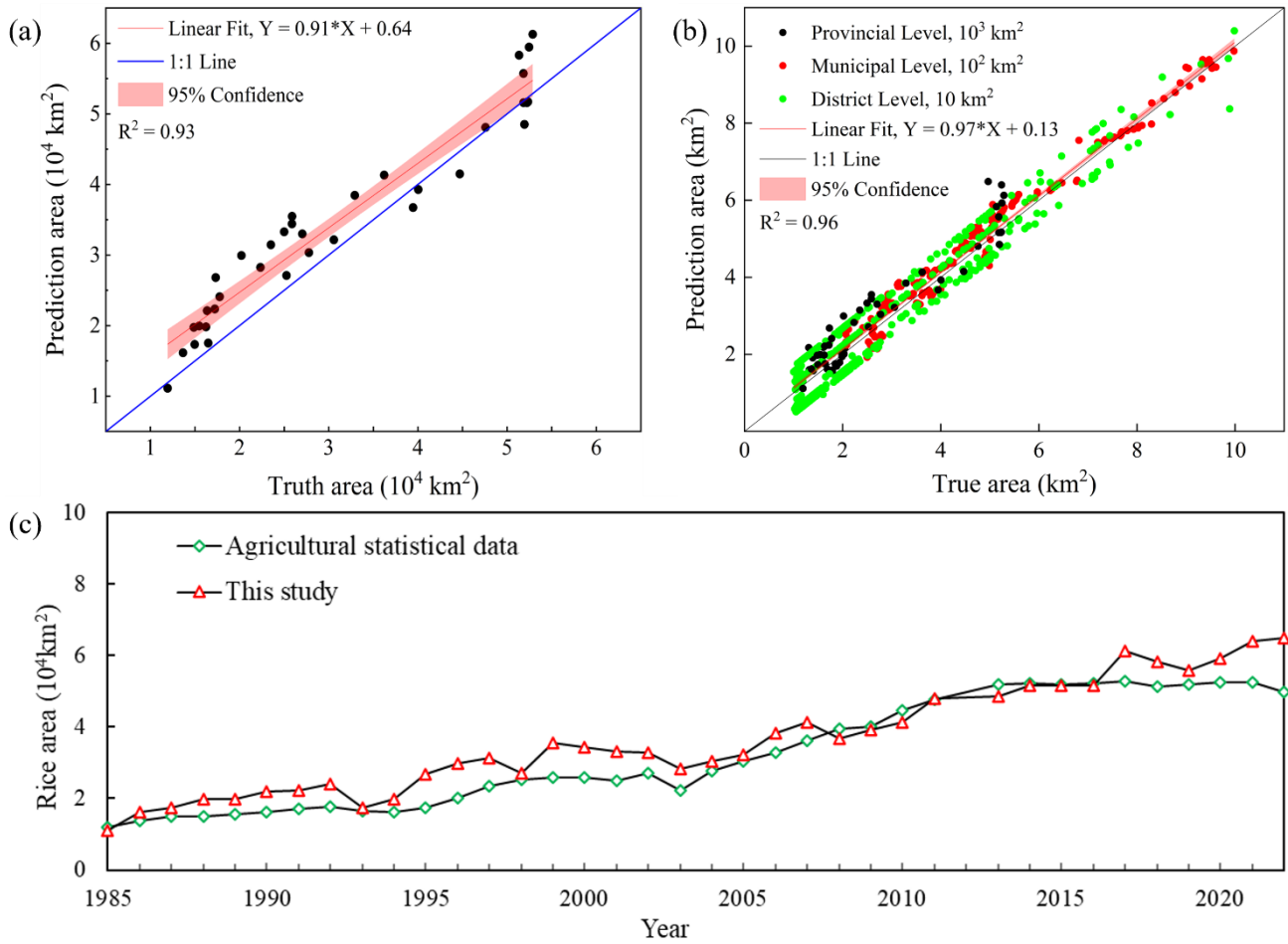
Figure 5: Comparison of paddy rice maps with agricultural statistical data. (a) presents the paddy rice area comparison across the entire study area. (b) is the comparison of the paddy rice area at provincial, municipal, and district levels within the study area. (c) shows the difference between the agricultural statistical data and the results of this study regarding paddy rice area estimation.
