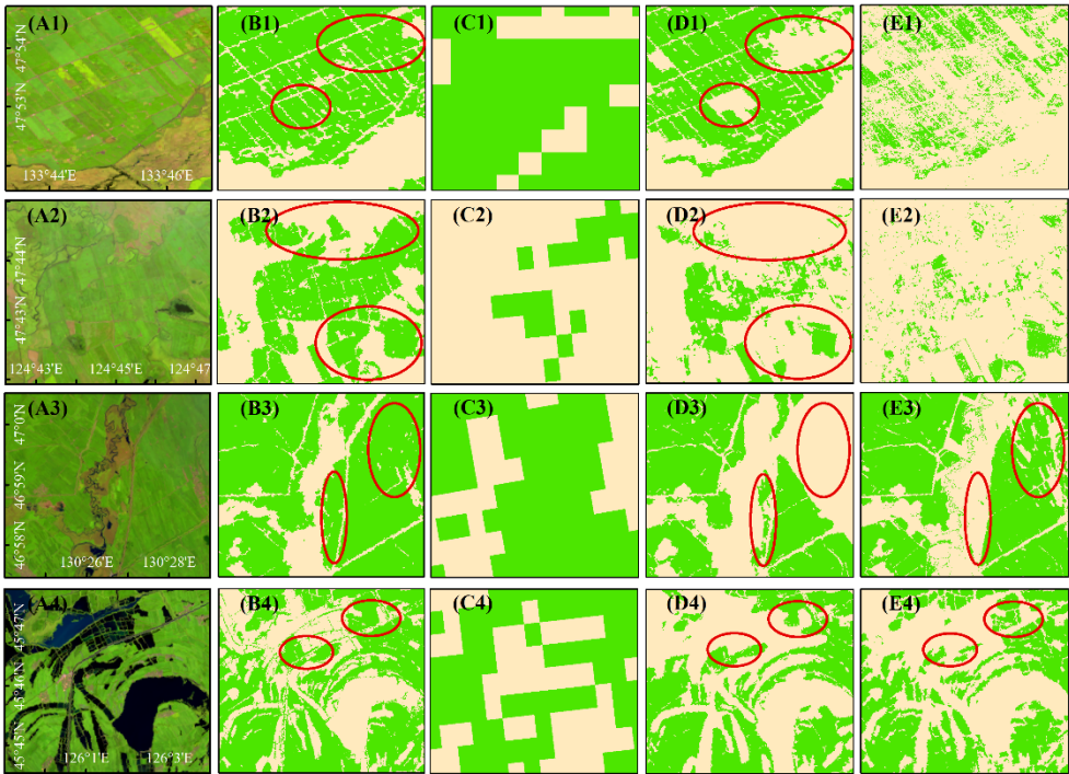
300 Figure 6: Comparison of the paddy rice products of this study with the existing products. (A1)-(A4) represents pseudo-colored (bands SWIR 1, NIR, and Red) of Landsat 8/9 images. (B1)-(B4) is the result of this study. (C1)-(C4) shows the paddy rice with MODIS data. (D1)-(D4) demonstrate the paddy rice with Landsat data. (E1)-(E4) depict the paddy rice maps using Sentinel-1 and Sentinel-2 images. The red circles indicate areas with significant differences in paddy rice.
