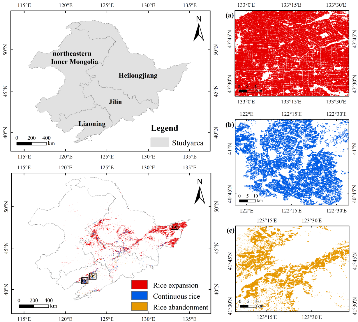
330 Figure 9: Trends of paddy rice cultivation area in Northeast China from 1985 to 2023.
