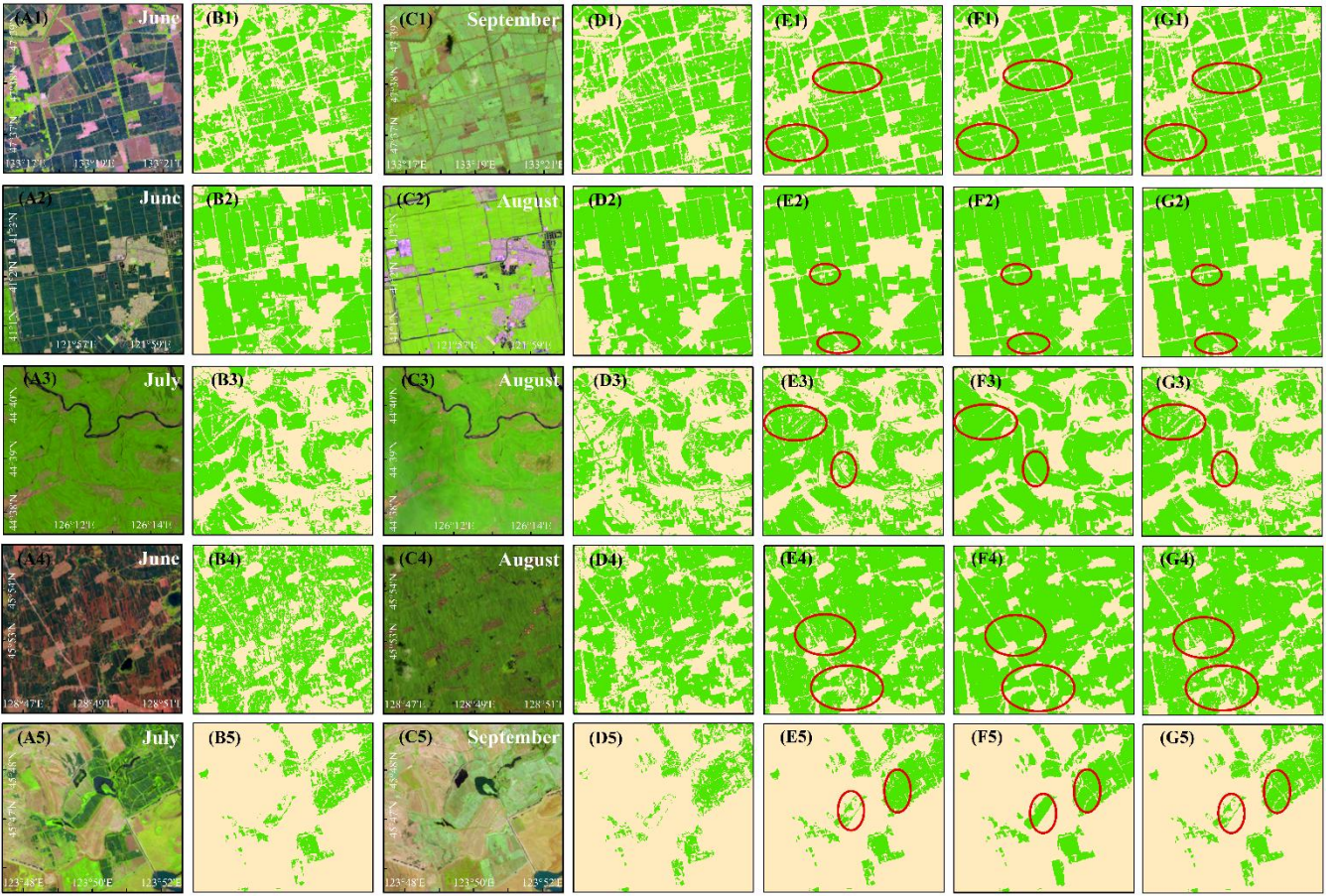
Figure 43: Comparison of paddy rice maps between ARE, single temporal, and overlay methods using Landsat 5 TM and Landsat 8 OLI images. (A1)-(A3), (C1)-(C3) represent pseudo-colored maps of three regions in the Landsat 8 images (bands SWIR 1, NIR, and Red6, 5, and 4 ) from June to September. (A4), (A5), (C4), and (C5) represent pseudo-colored maps of two regions in the Landsat 5 images (bands 5, 4, 3SWIR 1, NIR, and Red ) from June to September. B i (B1)-(B5) display the paddy rice maps corresponding to the images in A i (A1)-(A5) . (D1)-(D5) shows the paddy rice maps corresponding to the images in C i (C1)-(C5) . E i (E1)-(E5) are the overlay results of the paddy rice maps from columns A and C A i and C i . F i (F1)-(F5) depict ARE paddy rice maps obtained from all images available at that year . G i depict the ARE paddy rice maps from A i and C i , i \in [1,5] \cap \mathbb{Z} . The red circles in the overlay and ARE maps indicate areas with significant differences in paddy rice.
