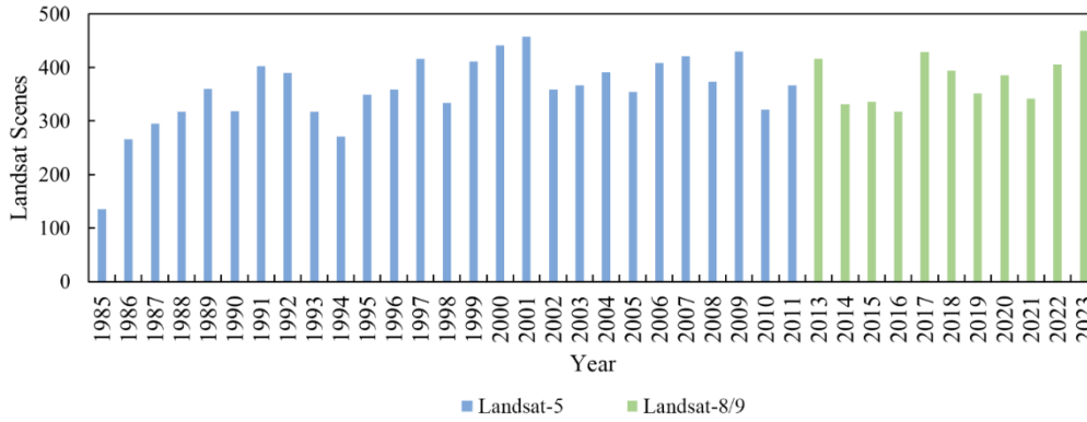
Figure 32: Number of Landsat images from 1985 to 2023 used in this study.
