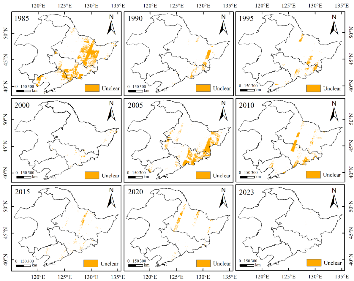
Figure 76: Areas lack at least one clean-sky observation during the annual growth stage of paddy.
