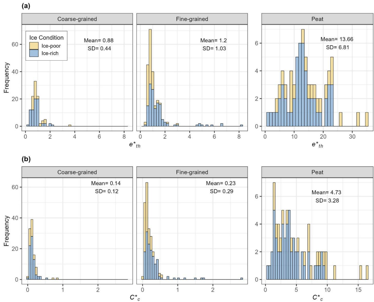
Figure 11: Frequency histograms of (a) threshold thawed void ratio ( e_{th}^* ) and (b) compressibility index of thawed soil ( C_c^* ) across three main soil categories. Different colors represent the ice conditions.
