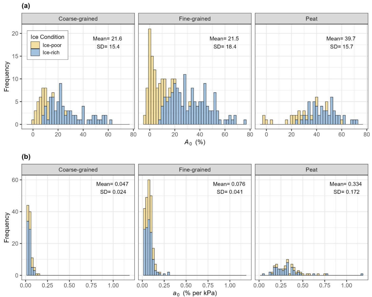
475 Figure 10: Frequency histograms of (a) the thaw strain parameter ( A_0 ) and (b) the coefficient of volume compressibility ( a_0 ) across three main soil groups. Different colors represent the ice conditions, highlighting the lower values of A_0 in ice-poor conditions compared to samples classified as ice-rich. For a_0 , both ice-rich and ice-poor samples exhibit similar ranges within each soil group; however, the mean value of a_0 is higher for peat compared to mineral soils, and for fine-grained soils compared to coarse-grained soils.
