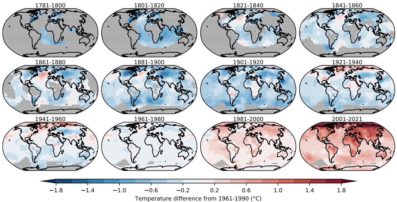
Figure 2. 20-year average SAT for the GloSATref analysis ( ^{\circ}\text{C} relative to 1961-1990, final panel shows 21-year average). Each panel averages available gridded data to quarterly, annual and then 20-year (21-year) averages, requiring data in at least two quarters to form an annual average and at least 10 annual averages to produce a 20-year average.
