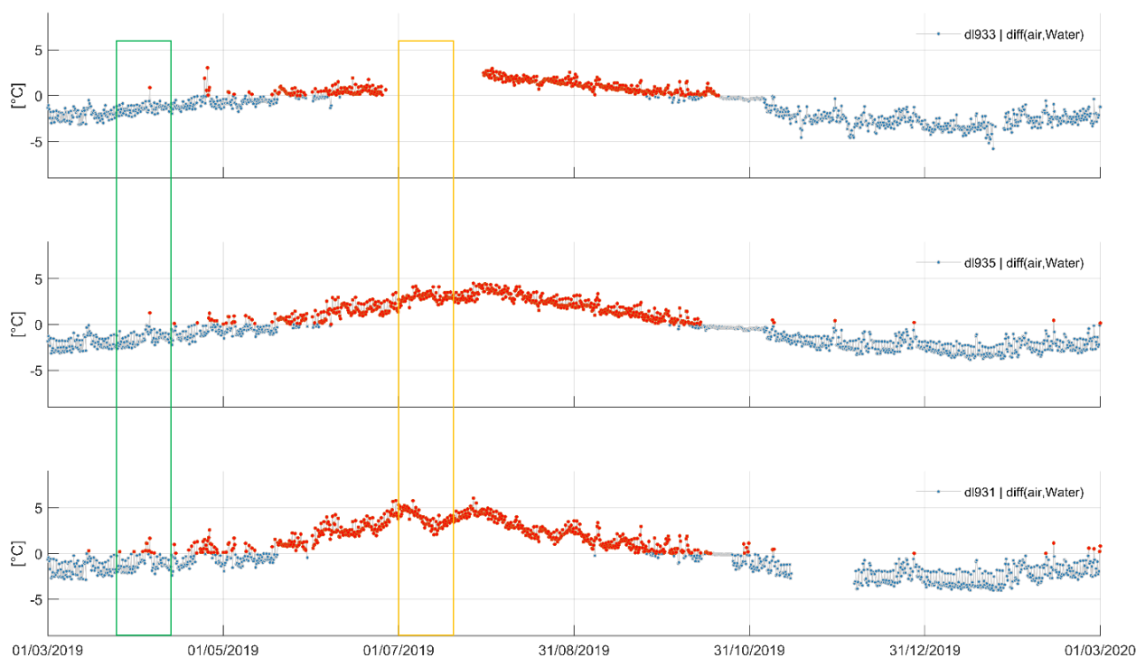
495 Figure 10: The difference between the sewer headspace temperature and the bulk liquid temperature observed at three specific locations in the main collector. Red dots indicate periods of evaporation (higher temperature in the headspace compared to the bulk liquid) and blue colours indicate periods of condensation (inverse temperatures). From the SI of Figuroa et al. (2022).
