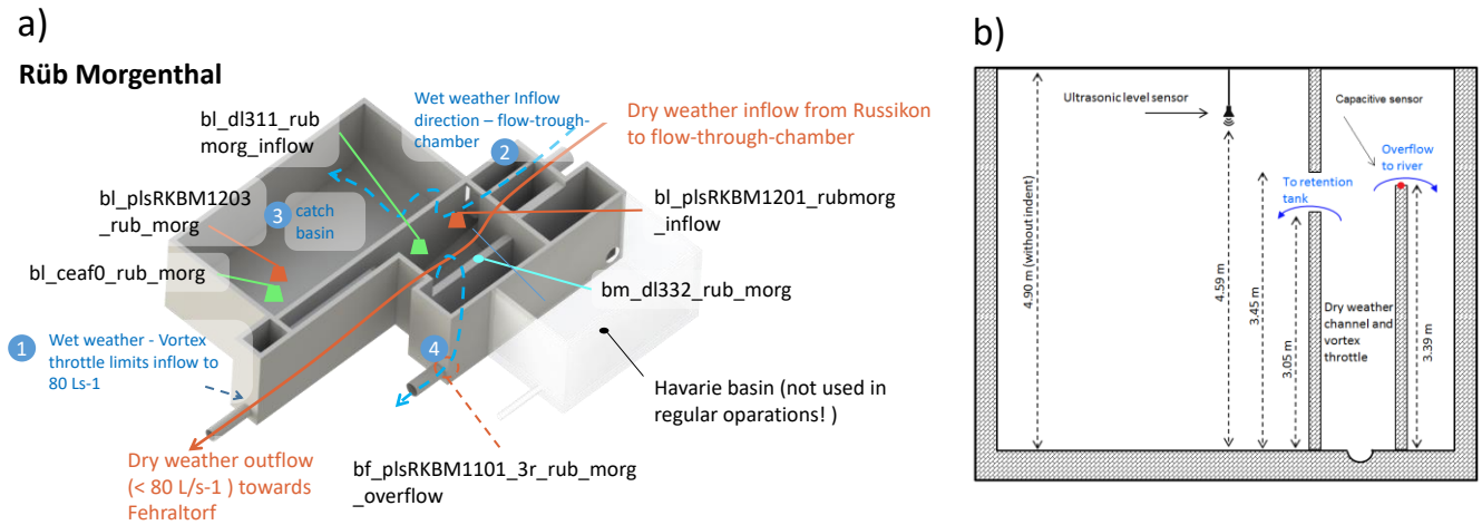
140 Figure 3a): CAD model of the overflow structure “RÜB Morgenthal” including inflow chamber, detention tank, overflow to receiving water, and installed sensors, b): Cross-section at the sensor bl_plsRKBM1201_rubmorg_inflow (not drawn to scale). Detailed information of all other detention basins and flow control structures is provided in the SI.
