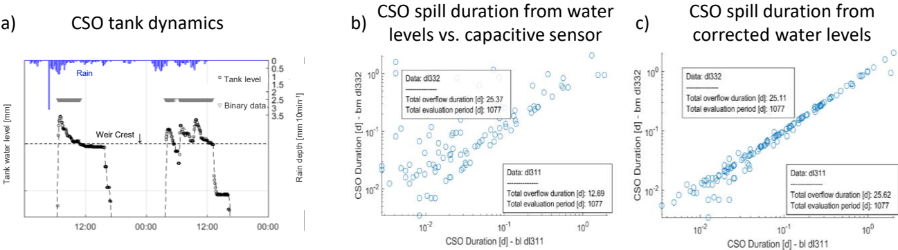
Figure 9a): Continuous tank level measurements (dots) and binary data (triangles). The latter are derived from the capacitive sensor signal, reflecting an overflow activity during a period of two days for which two independent overflow events were recorded, b) and c): Event-specific overflow durations derived from one capacitive sensor (bm_dl332_rub_morg) and one ultrasonic level sensor (bl_dl311_rubmorg_inflow). The overflow duration derived from the erroneously calibrated level sensor (dl311) with an incorrect offset in b) is corrected to a correct offset in c). 555
