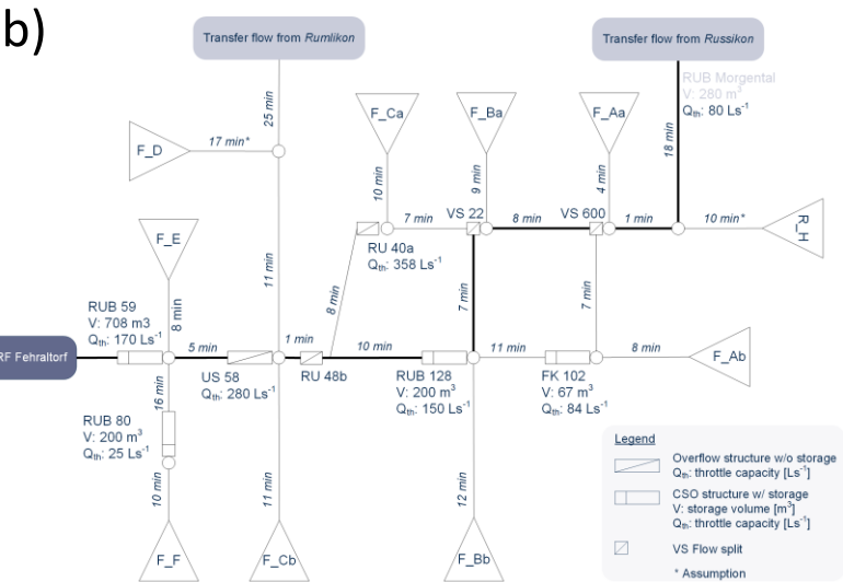
Figure 2a): Overview of the Fehraltorf catchment, including urban drainage network, geography and land use. b): Simplified flow scheme of the combined sewer system of Fehraltorf. The main flow path through the network is from top right to the left (bold line). The relevant characteristics of sub-catchments can be found in the supporting information. Indicated flow times are calculated assuming a constant flow velocity in the sewer of 1 ms -1 .
