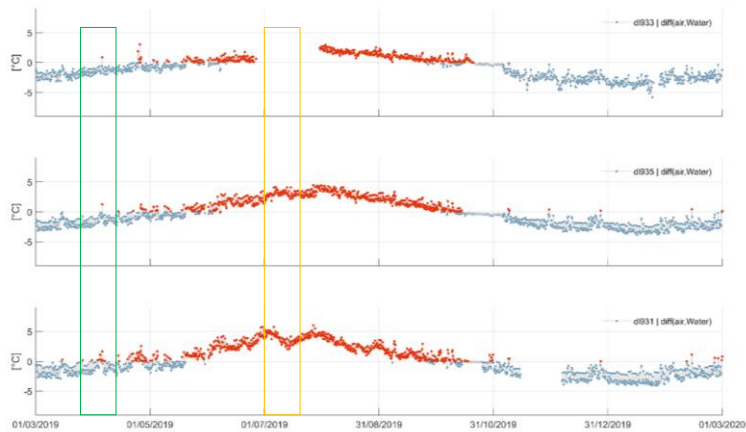
Figure 10: The difference between the sewer headspace temperature and the bulk liquid temperature observed at three specific locations in the main collector. Red dots indicate periods of evaporation (higher temperature in the headspace compared to the bulk liquid) and blue colours indicate periods of condensation (inverse temperatures). From the SI of Figueroa et al. (2022).
