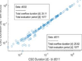
CSO spill duration from corrected water levels
