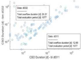
b) CSO spill duration from water levels vs. capacitive sensor
