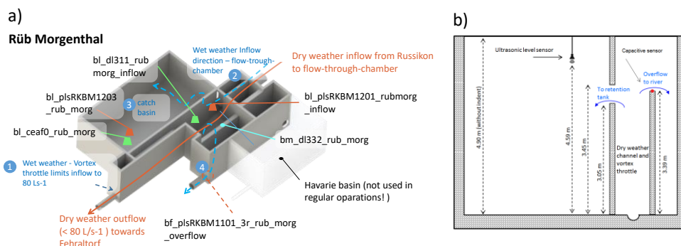
Figure 3 left: CAD model of the combined-sewer-overflow (CSO) tank “RUB Morgenthal” including inflow-chamber, detention tank, overflow to receiving water and installed sensors. Right: Cross-section through the overflow structure at the sensor bl_plsRKB1201_rubmorg_inflow (not drawn to scale). Detailed information of all detention-basins and flow-control-structures is provided in the SI-a); CAD model of the overflow structure “RÜB Morgenthal” including inflow chamber, detention tank, overflow to receiving water, and installed sensors. b): Cross-section at the sensor bl_plsRKB1201_rubmorg_inflow (not drawn to scale). Detailed information of all other detention-basins and flow-control-structures is provided in the SI.
