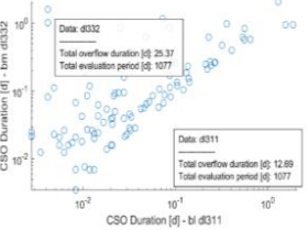
CSO spill duration from water levels vs. capacitive sensor
