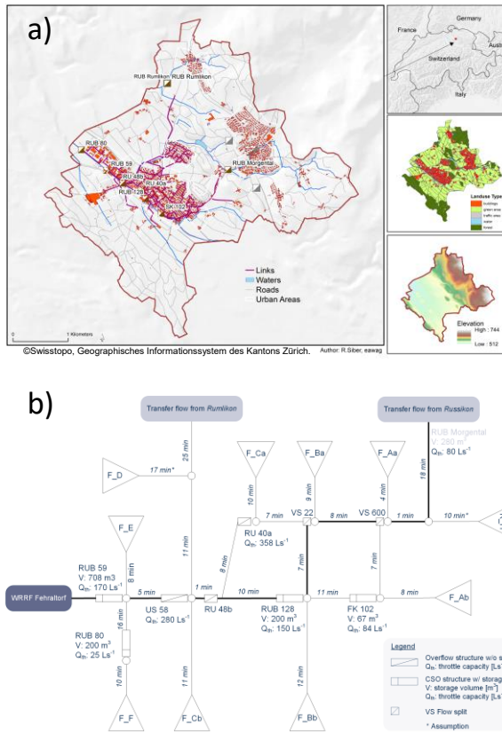
Figure 2a)–Top: Overview of the Fehraltorf catchment, including urban drainage network, geography and land use. Bottomb): Simplified flow scheme of the combined sewer system of Fehraltorf. The main flow path through the network is from top right to the left (bold line). The relevant characteristics of sub-catchments can be found in the supporting information. Indicated flow times are calculated assuming a constant flow velocity in the sewer of 1 ms -1 . The urban drainage flow scheme of Fehraltorf, illustrating the combined-sewer network of Fehraltorf. The main flow path through the network is from top right to the left (bold line). Triangles represent aggregated sub-catchments. The relevant characteristics can be found in the supporting information. The here indicated flow-times are estimated assuming a flow-velocity in the sewer of 1 ms -1 .
