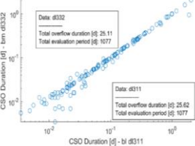
c) CSO spill duration from corrected water levels
