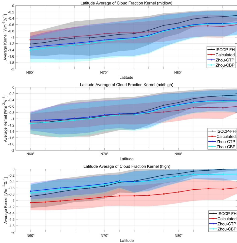
Figure 10. Comparison of latitudinally weighted means for the ISCCP-FH CRKs, Zhou-CTP/CBP CRKs and GCF-CRKs in the different cloud layers
