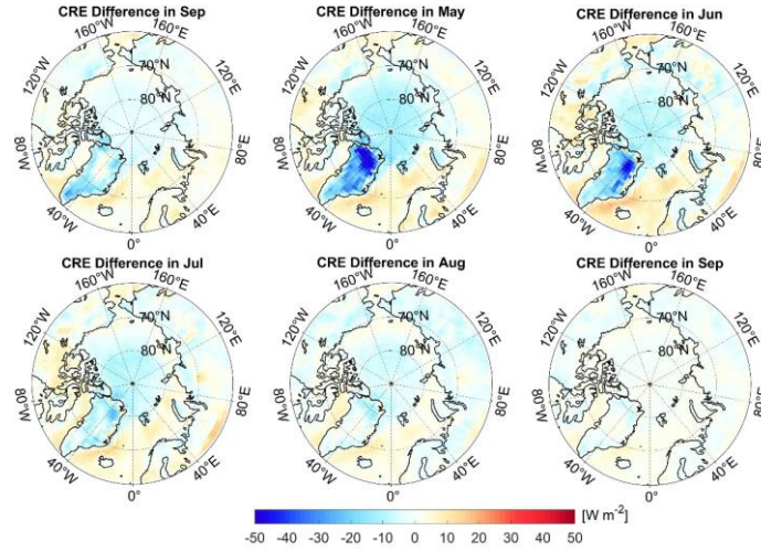
Figure 12. Spatiotemporal distribution for the surface SW CRE differences. The CRE calculated from the GCF-CRKs minus the CRE derived from the CERES-EBAF DSSR data.
