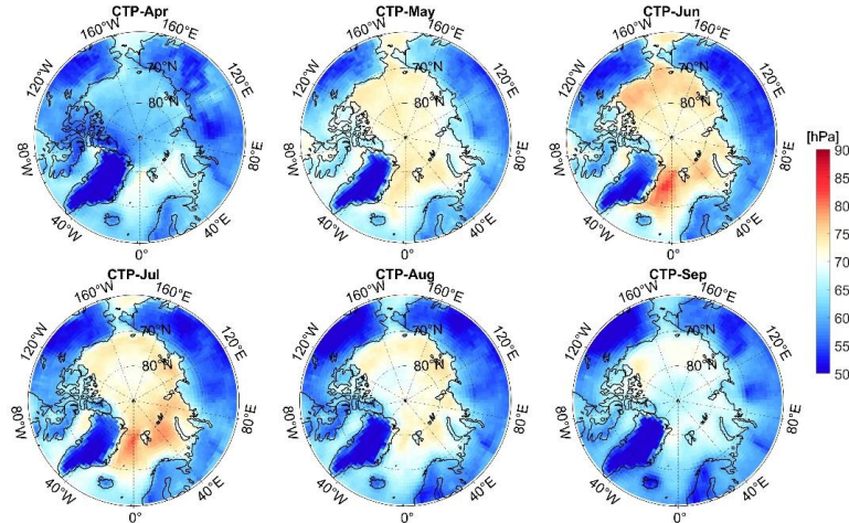
Figure A3. The average monthly cloud top pressure (CTP) in the Arctic from April to September, 2000-2020
