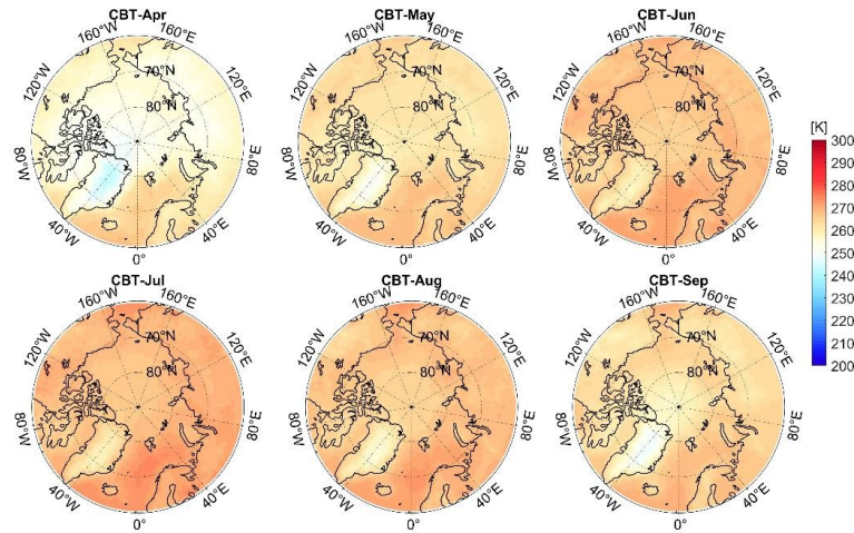
Figure A6. The average monthly cloud base temperature (CBT) in the Arctic from April to September, 2000-2020
