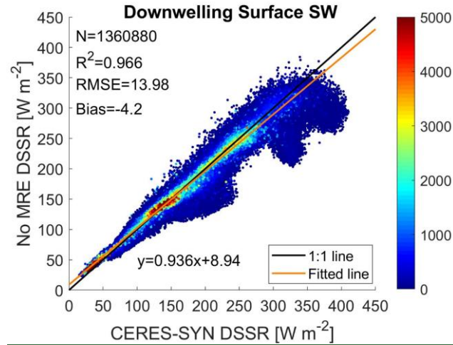
Figure 156 Scatter plot comparing the DSSR estimated without considering multiple reflection effects (MRE) and the CERES-SYN1deg DSSR.
