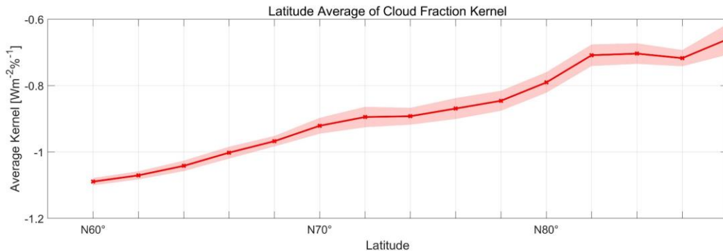
Figure 1617. Latitude-weighted mean of the deseasonalized grid-based surface cloud fraction cloud radiative kernels (SFC GCF-CRKs)
