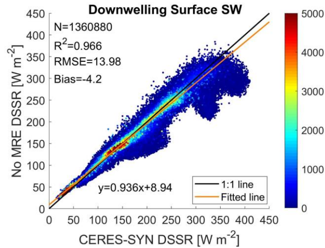
Figure 15 Scatter plot comparing the DSSR estimated without considering multiple reflection effects (MRE) and the CERES SYN1deg DSSR.
