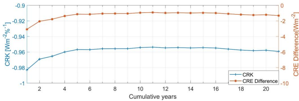
Figure 1718. Differences in the grid-based surface cloud fraction radiative kernels (SFC GCF-CRKs and in the CRE) estimated using data with varying time lengths.
