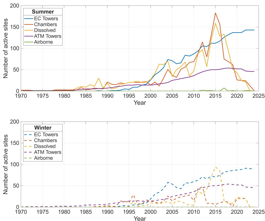
Figure 3. Cumulative temporal coverage of all available sites/studies shown separately for each observational platform. Measurement platforms are abbreviated as stated in Table 1. Please note that for EC and ATM towers, sites are considered to be operational until discontinuation is indicated by the operators, therefore data coverage remains high for these categories also in recent years. For all other categories, data availability relies on results or data being published, therefore time lags between measurement and being listed in this database lead to declining data coverage for the past decade. A distinction is made between summer (top) and winter activity (bottom). In cases where seasonal activity data are not available, only summer activity is assumed, except for atmospheric towers which are assumed to be active throughout the year.
