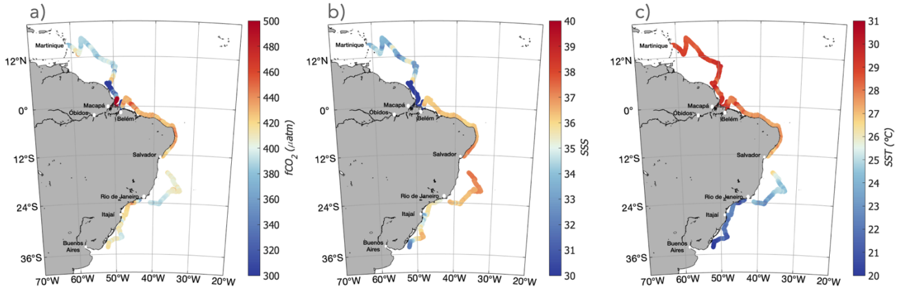
Figure 5: Along track a) \text{CO}_2 fugacity (complete range of values shown in Figure 4), b) sea surface salinity and c) sea surface temperature.
