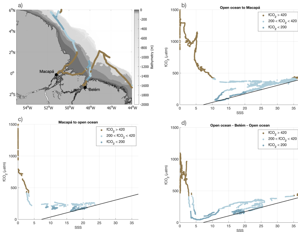
Figure 8: a) Map of the Amazon region, with bathymetry contours. Each region is defined on Figure 9. The track is colored based on the f\text{CO}_2 values to highlight three regimes ( f\text{CO}_2 \geq 420 \mu\text{atm} (brown), 200 \mu\text{atm} < f\text{CO}_2 < 420 \mu\text{atm} (light blue) and f\text{CO}_2 \leq 200 \mu\text{atm} (dark blue)). f\text{CO}_2 -SSS diagram for the entrance in the Amazon River (b) for the exit of the Amazon River (c) and for the sampling of the Pará River (d). The black line on b) c) d) is the f\text{CO}_2 /SSS relationship from Lefèvre et al., (2010).
