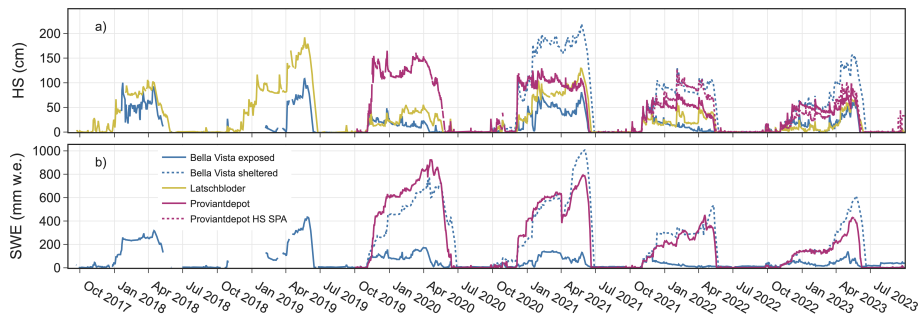
Figure 7. Daily averaged HS (a) and SWE (b) measurements (Oct-September 2017 to Aug-August 2023) at the three stations Bella Vista, Latschbloder and Proviantdepot.
