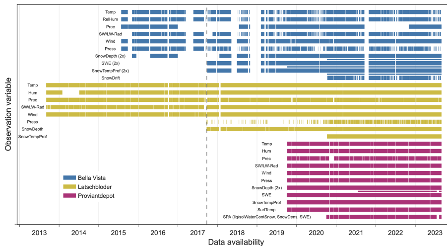
Figure 4. Data availability for the three AWSS Bella Vista, Latschbloder, and Proviandtepot for all measured variables 2013 to 2023. Narrow Some variables are recorded with two different sensors at the same location. These are indicated by (2x) and the narrow bars indicate a show the data availability for the second sensor for a variable. The vertical dashed line highlights the beginning of the data period presented here (September 2017). The plot is based on daily aggregations of the data. If one 10 min value is missing on a specific day, the entire day is classified as missing data in this figure. The frequent short gaps in atmospheric pressure readings at the Bella Vista and Latschbloder site are caused by frequent single 10 min data points missing (unidentified malfunction of the logger). The large data gaps at the Bella Vista station were caused by recurring lightning damage.
