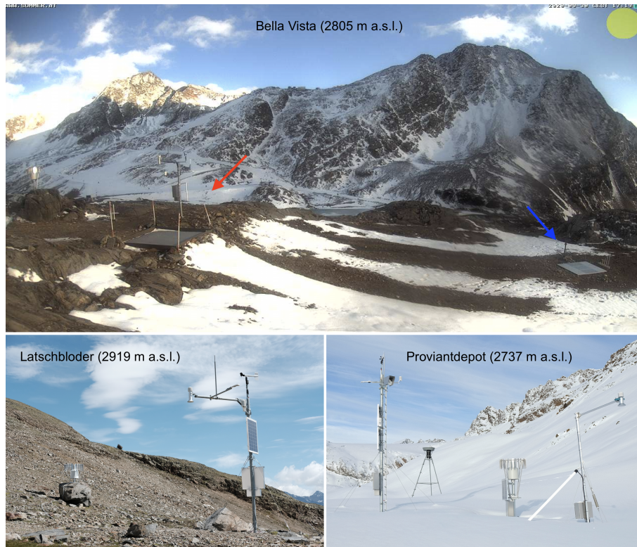
Figure 2. Webcam-Top: webcam image from the Bella Vista station (top2805 m a.s.l.). The red arrow marks the main “exposed” AWSS. The blue arrow marks the additional snow measurements (HS, SWE, and snow temperatures) in the slight depression (“sheltered” location). Bottom left: the Latschbloder AWSS (2919 m a.s.l.) with an Ott Pluviometer on the left. Bottom right: the Proviantdepot AWSS (2737 m a.s.l.). The ultrasonic snow depth sensor on the right instrument is part of the Snow Pack Analyzer (SPA). The snow scale is buried right in front of the photographer besides the SPA. There is a second snow depth sensor at the main mast (not visible from this angle). Behind the main mast the old totalizing rain gauge can be seen, and in the background the Kesselwandferner (left, behind the main mast).
