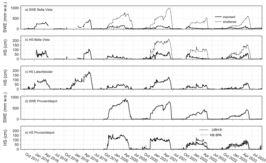
Figure 6. Measured SWE and HS (where available) at the Bella Vista double snow station setup (a and b), at the Latschbloder (c) and Proviantdepot (d and e) stations from Oct-September 2017 to Aug-August 2023.
