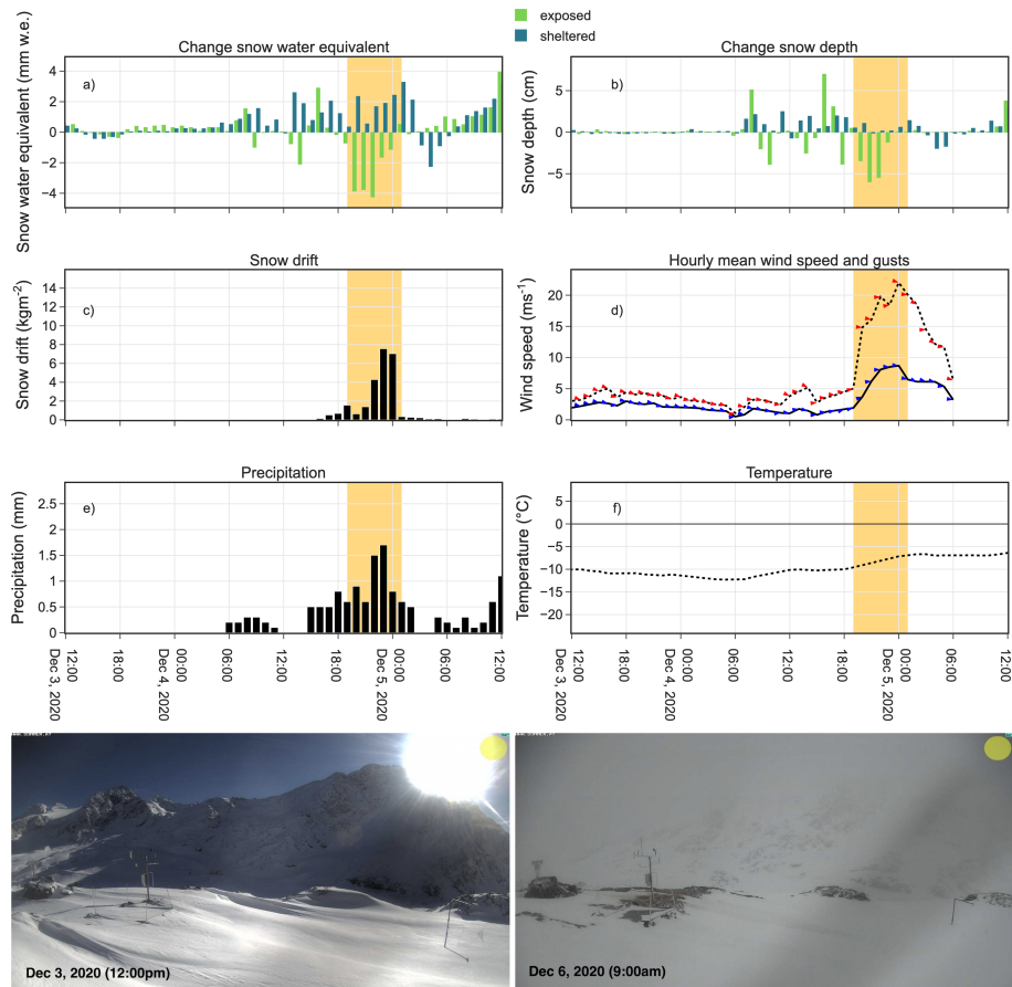
Figure 11. Measurement of a snow drift event at the Bella Vista station -Data from Dec 3, 2020 (12:00 pm) to Dec 5, 2020 (12:00 pm): hourly data of changes in SWE (a) and HS (b) each at the exposed and sheltered location, snow drift (c), wind speed and gusts (d), precipitation (e), and air temperature (f). Wind directions for mean wind and gusts are indicated by blue and red arrows, respectively in (d). The period of the main blowing snow event is highlighted in yellow. The webcam images are taken before (left, Dec 3, 12:00 pm) and shortly after a blowing snow event (right, Dec 6, 2020, 9:00 am). The main AWSS (exposed location) can be identified in the left side of the pictures, the complementing, second SWE and HS measurements are located at the mast on the right side in the pictures (sheltered location).
