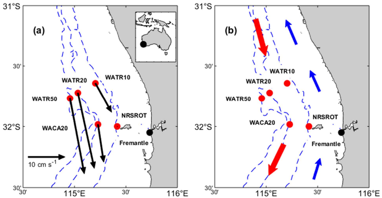
Figure 1. Bathymetry map and mooring locations (red circles) on the Rottneest Shelf. (a) Velocities estimated from measurements, with black arrows representing the mean state of vertically averaged velocities. The 0-200m average is used for the WATR50 mooring. The three dashed lines represent the 50m, 200m, and 500m contours. Black circles indicate the location of the Fremantle tide gauge station. Note that NRSROT consists of two separate moorings. (b) Schematic of shelf currents systems, with red arrows denoting the Leeuwin Current and blue arrows indicating the direction of the wind-driven Capes Current.
