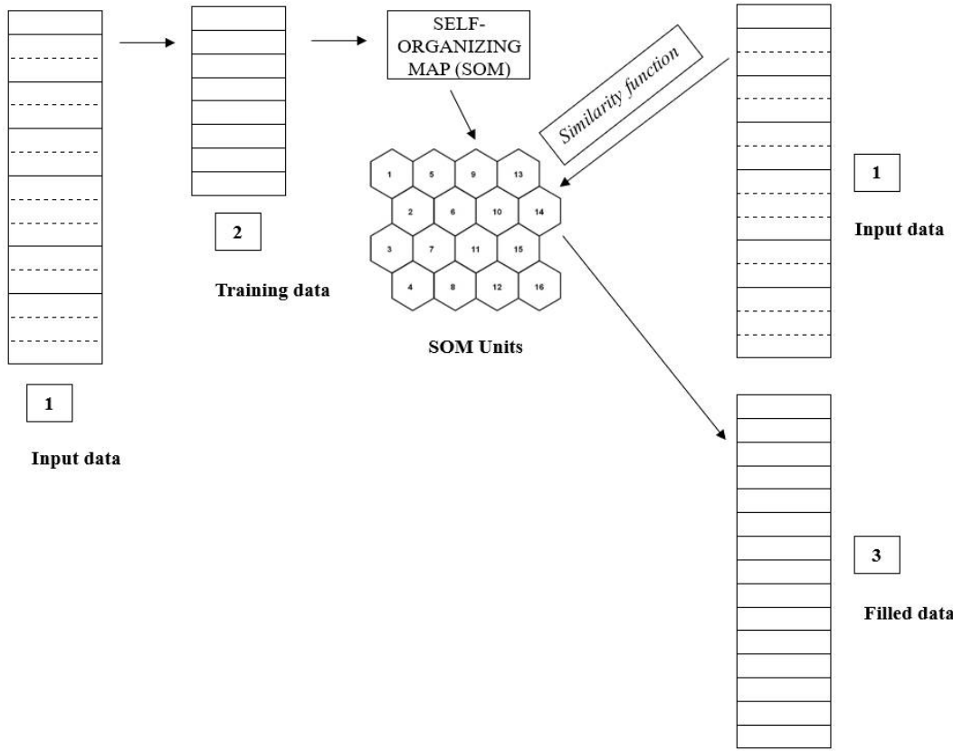
Figure 2. Schematic of the SOM method applied to fill gaps in the mooring temperature and velocity data. Square-Dataset 1 denotes an input data matrix in which rows are daily time vectors, columns are observational variables. In square-Dataset 1 , solid lines present full available profiles, while dashed lines show the profiles including missing values. In square-Dataset 2 , only full data profiles are selected for training in SOM. In SOM, we pre-define the number of units, for instance 1000 units for temperature, and 500 units for velocity. Each SOM unit contains a reference vector. On the right hand side, each daily input vector in the input data matrix is assigned to each SOM unit using a similarity function defined by Chapman and Charantonis, 2016. Finally, we use the referent vector of each SOM to fill gaps in corresponding daily input vector, shown in square-Dataset 3 .
