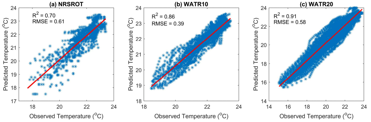
Figure 3. Scatter plots of observed and estimated-SOM-derived temperatures at the three moorings between 1/1/2020 and 30/5/2020, a period of 150 days. The red lines are the line of best-linear fits of the scatter plots.
