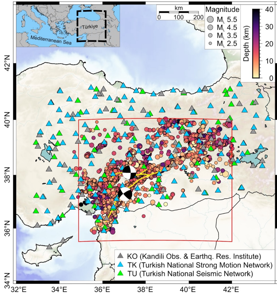
Figure 1: The data set for the East Anatolian Fault Zone (EAFZ) described in this work, bounded by the red box (Lon-Lat vertices, SW: 34.89 35.50; SE 42.00 35.50; NE 42.00 40.00; NW: 34.89 40.00). Dots represent the events with M_L between 2.0 and 5.5 in the period 01-01-2019 to 29-02-2024. The size is proportional to the magnitude; the color palette represents the event depth. The two beach balls lying in the Melgar faults (yellow lines) represent the Mw 7.8 Pazarcık earthquake and the Mw 7.6 Elbistan earthquake occurred on February 6, 2023, which are not considered in this catalog. The triangles show the different networks that recorded the events: KO (gray), TK (cyan) and TU (green).
