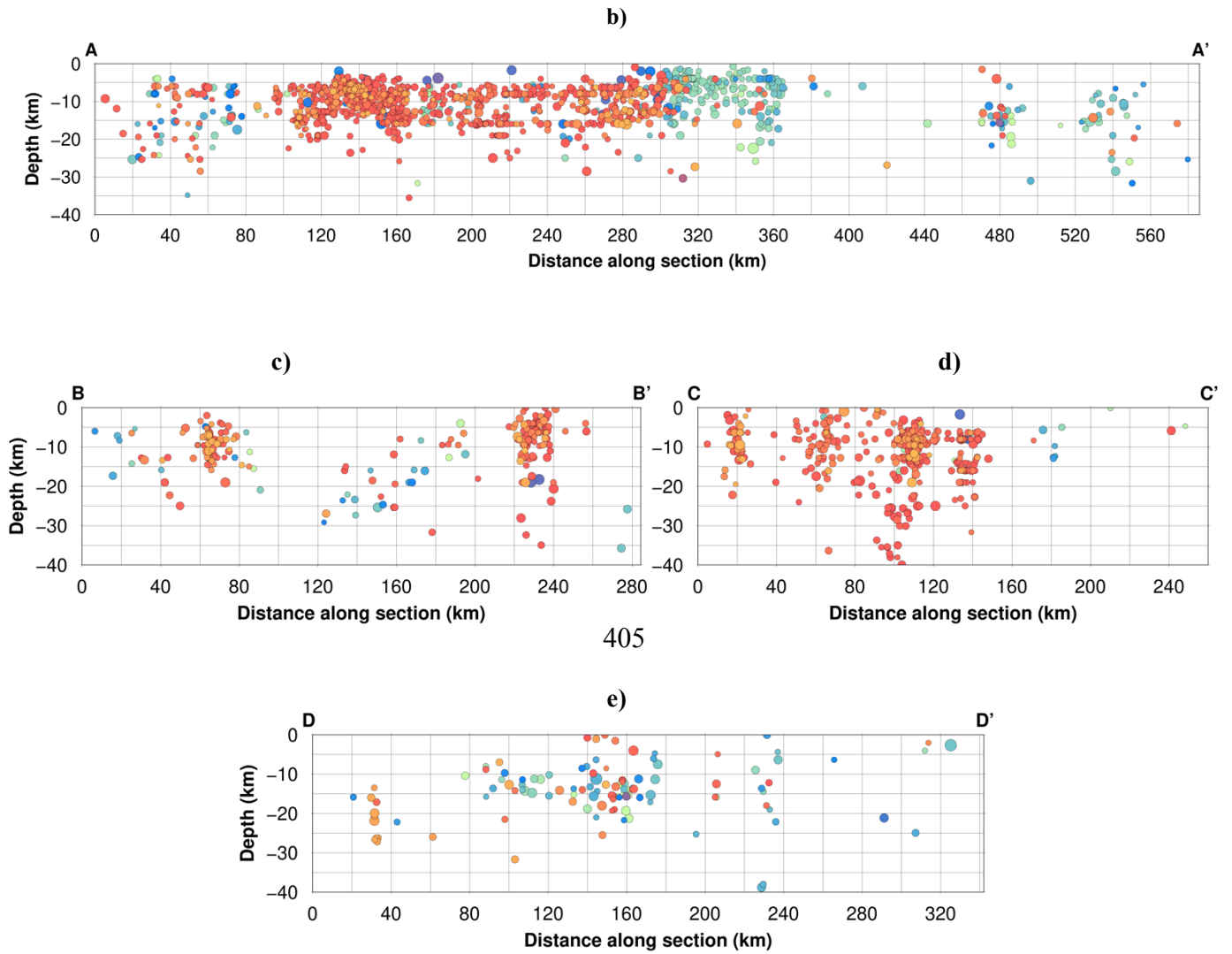
410 Figure 14: a) Seismicity map of the distributed catalog. The color scale represents the temporal evolution of the seismicity, while the size of the point is proportional to the magnitude. In red is shown the rectangle surrounding the study area, in yellow we show the faults according to Melgar et al. (2023) . Profiles are shown with black lines. b) Section A-A', length 586 km, 1303 events. c) Section B-B', length 284 km, 202 events. d) Section C-C'; length 260 km, 433 events. e) Section D-D'; length 342 km, 118 events. 415 Each profile was performed considering the events 10 km further to the left and 10 km to the right with respect to the line track. Vertical exaggeration of the cross-sections is 2:1.
