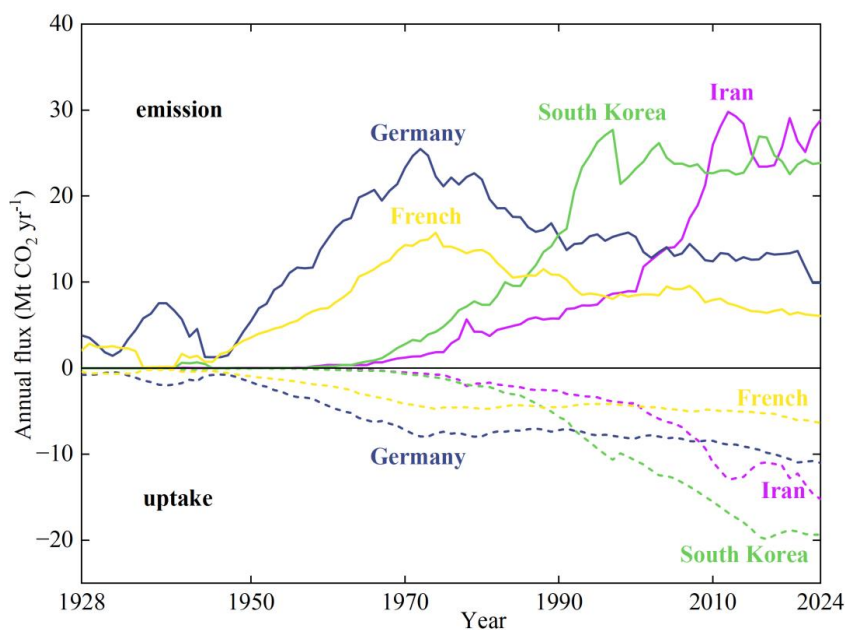
355 Figure 5: Comparison of trends of carbon emission and uptake in peaked and non-peaked countries.
