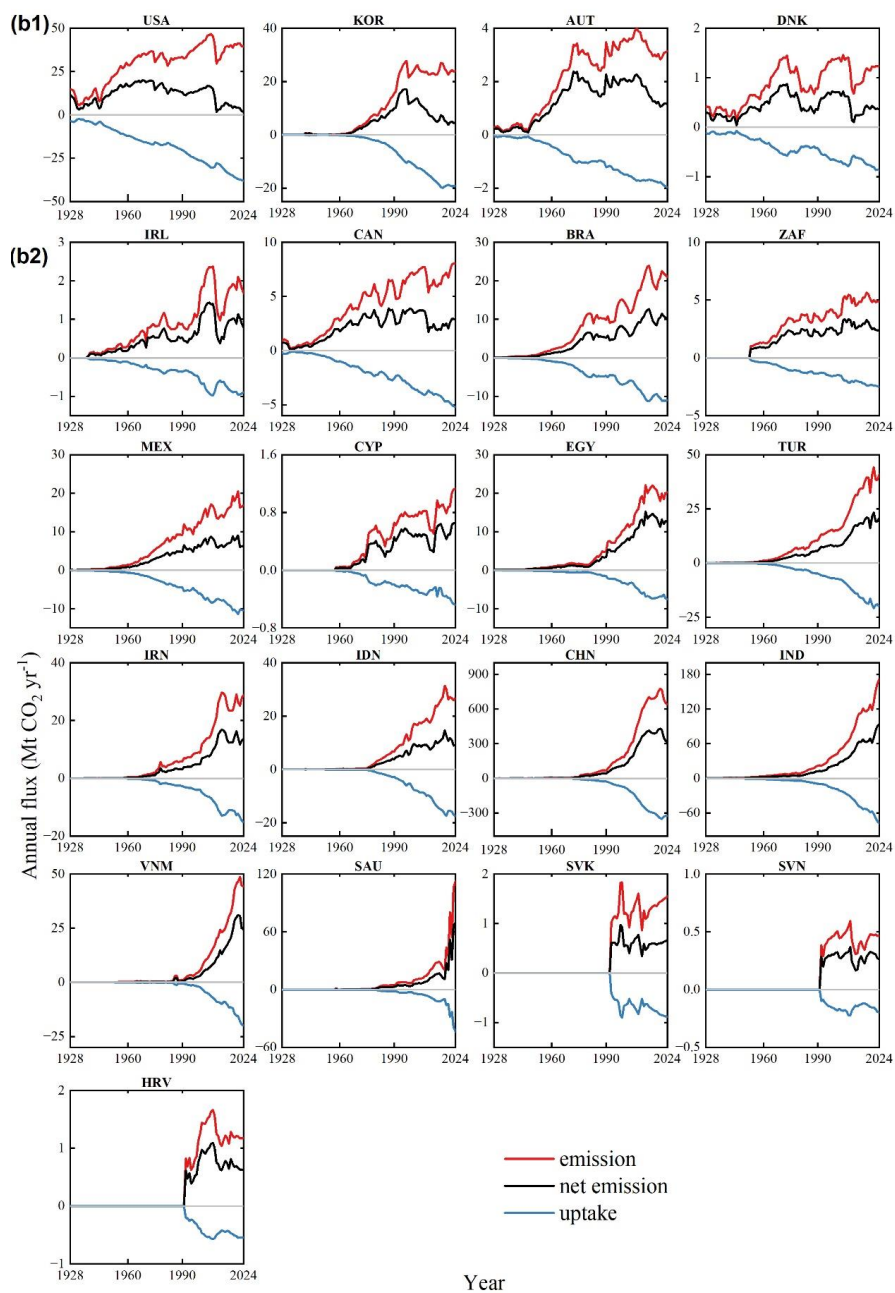
Figure 4: Cement carbon emission and uptake in 42 countries during 1928-2024. (a) 21 countries in Group 1 that the cement process emissions have reached peaking. (b) 21 countries in Group 2 with carbon emissions non-peaked.
