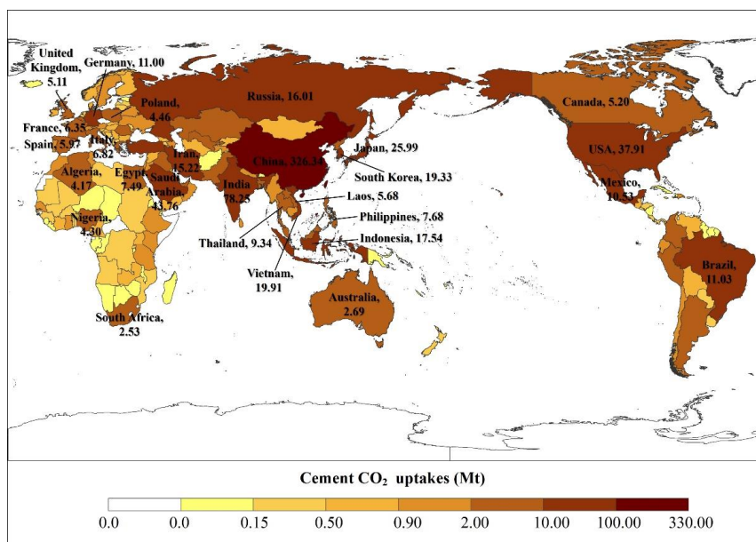
300 Figure 3: Spatial distributions of cement CO 2 uptake in 2024. (The map is copyrighted by the Institute of Geographic Sciences and Resources of the Chinese Academy of Sciences, with no modifications to the base map)
