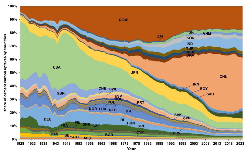
280 Figure 2: Share of cement carbon uptake from 1928 to 2023 by 42 countries and rest of world (ROW). The full names corresponding to the country abbreviations are as follows: AUS (Australia), AUT (Austria), BEL (Belgium), BGR (Bulgaria), CAN (Canada), HRV (Croatia), CYP (Cyprus), CZE (Czechia), DNK (Denmark), FIN (Finland), FRA (France), DEU (Germany), GRC (Greece), HUN (Hungary),
