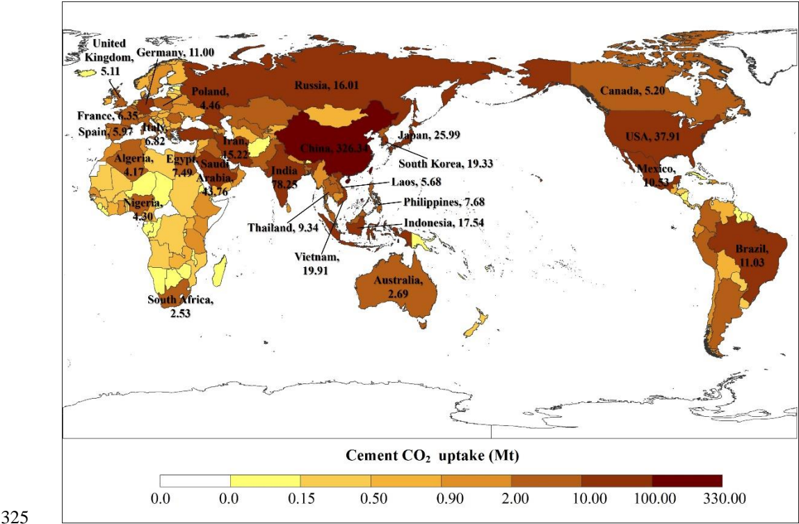
Figure 4: Spatial distributions of cement CO 2 uptake in 2024. (The map is copyrighted by the Institute of Geographic Sciences and Resources of the Chinese Academy of Sciences, with no modifications to the base map)
