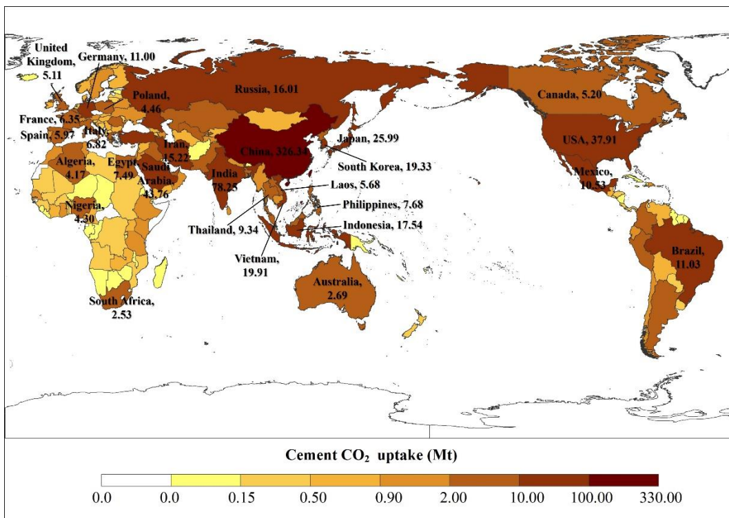
325 Figure 4: Spatial distributions of cement CO 2 uptake in 2024. (The map is copyrighted by the Institute of Geographic Sciences and Resources of the Chinese Academy of Sciences, with no modifications to the base map)
