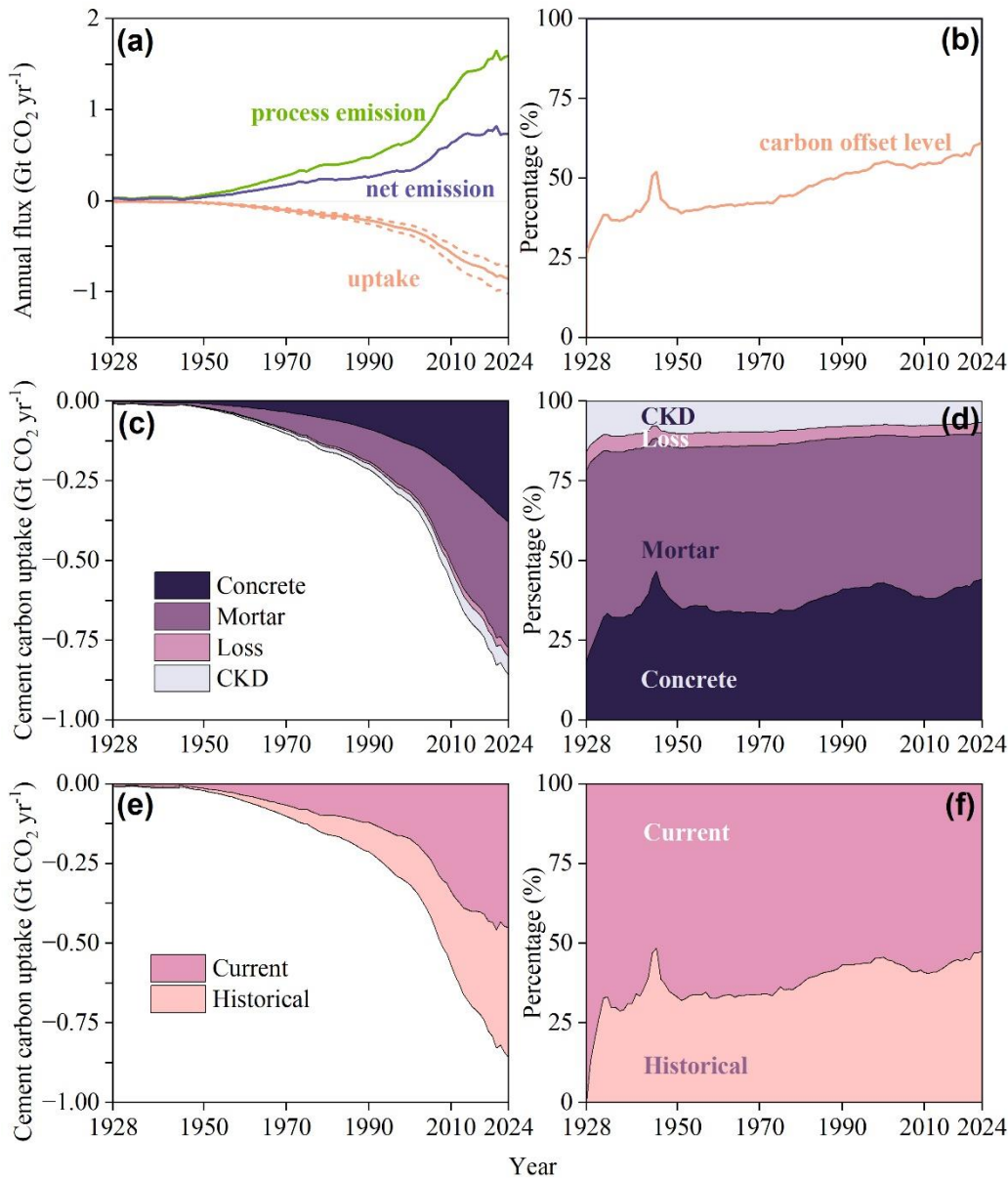
Figure 1: Global cement CO 2 uptake. (a) global annual process CO 2 emission and uptake by cement. (b) carbon offset level (share of CO 2 uptake to emission). (c) global annual CO 2 uptake by four cement material. (d) share of CO 2 uptake by four cement materials. (e) global cement annual CO 2 uptake in current and historical year. (f) share of CO 2 uptake by current and historical. The detailed results data are in Supplementary table 3 (available from https://doi.org/10.5281/zenodo.13827861 Wu et al., 2024).
