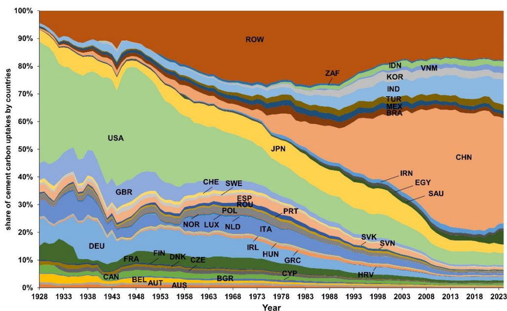
Figure 2: Share of cement carbon uptake from 1928 to 2023 by 42 countries and rest of world (ROW). The full names corresponding to the country abbreviations are as follows: AUS (Australia), AUT (Austria), BEL (Belgium), BGR (Bulgaria), CAN (Canada), HRV (Croatia), CYP (Cyprus), CZE (Czechia), DNK (Denmark), FIN (Finland), FRA (France), DEU (Germany), GRC (Greece), HUN (Hungary), IRL (Ireland), ITA (Italy), LUX (Luxembourg), NLD (Netherlands), NOR (Norway), POL (Poland), PRT (Portugal), ROU (Romania), SVK (Slovakia), SVN (Slovenia), ESP (Spain), SWE (Sweden), CHE (Switzerland), GBR (United Kingdom), USA (USA), MEX (Mexico), BRA (Brazil), EGY (Egypt), TUR (Turkey), IRN (Iran), SAU (Saudi Arabia), IND (India), CHN (China), KOR (Korea, Republic of), JPN (Japan), VNM (Vietnam), IDN (Indonesia), ZAF (South Africa).
