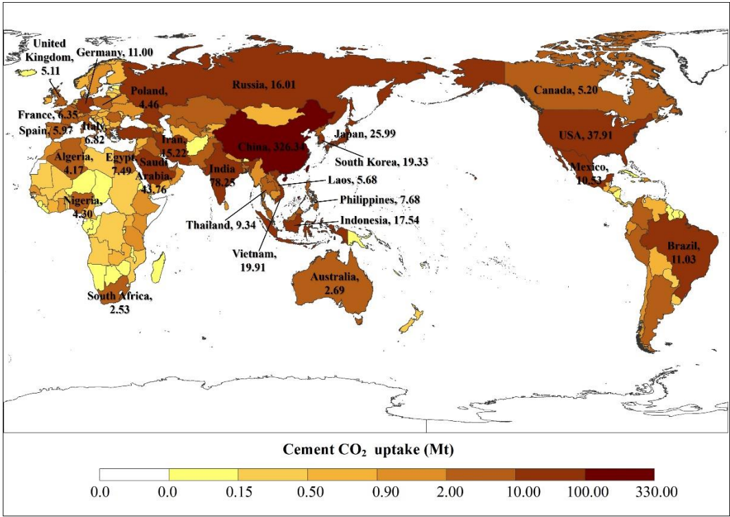
Figure 3: Spatial distributions of cement CO 2 uptake in 2024. (The map is copyrighted by the Institute of Geographic Sciences and Resources of the Chinese Academy of Sciences, with no modifications to the base map)
