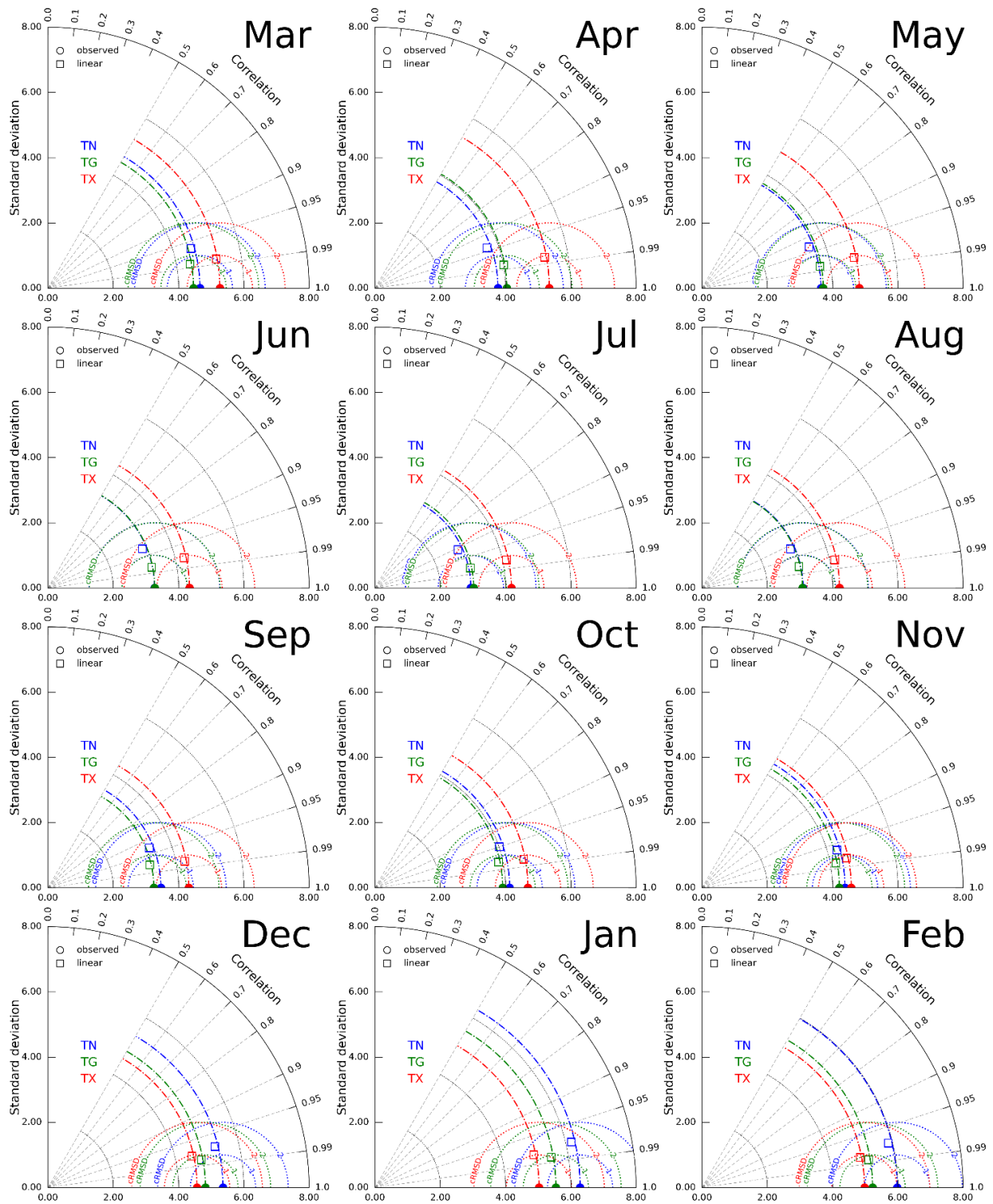
225 Figure 4. Taylor diagrams for LOO-CV of spatial interpolation of TN, TG and TX by linear RBF function. See Figure 3 for more details.
