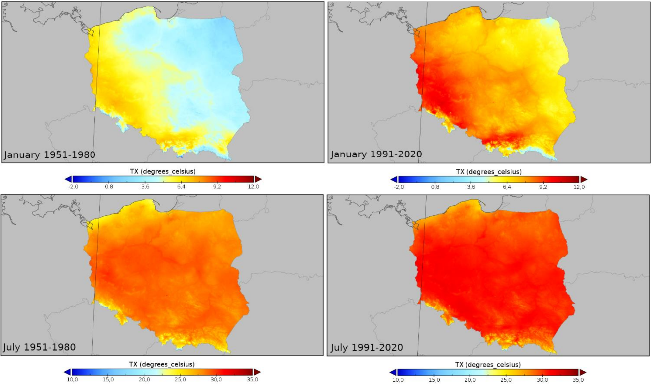
290 Figure 6. Spatial variability of the 90th quantile of TX in Poland for selected 30-year periods (1951-1980 left panel, 1991-2020 right panel) in January (upper panel) and July (lower panel).
