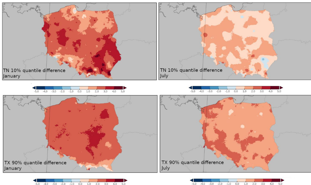
Figure 8. January (left) and July (right) differences ( ^{\circ}\text{C} ) between the values of TN 10th quantile (upper panel) and TX 90th quantile (lower panel) between periods 1991-2020 and 1980- 1951
