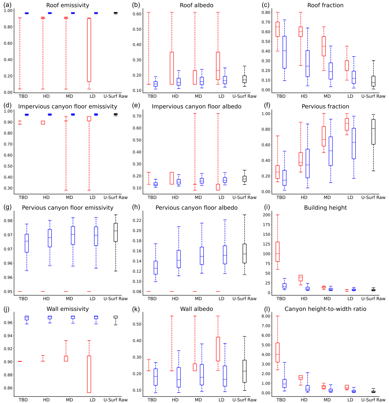
Figure 3. Distribution of urban surface properties at four density classes locations (Oleson and Feddema, 2020): Tall Building District (TBD), High Density (HD), Medium Density (MD), and Low Density (LD), compared with raw U-Surf data. Red bars represent CLMU values (discrete, 33 regions), and blue bars show new U-Surf values (continuous, 1 km) extracted from grids identified as TBD, HD, MD and LD per J2010's definition. The black bars show the distribution of 1 km U-Surf raw data. Box and whisker plots show the 25th, median and the 75th (the bottom, middle and top horizontal bars), and extend to the 5th and 95th quantiles.
