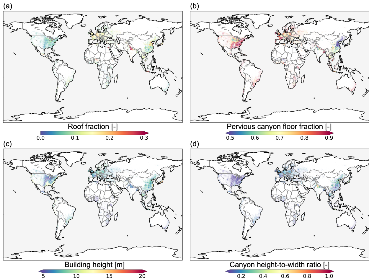
Figure 5. Global spatial distribution of U-Surf morphological parameters. (a) roof fraction [unitless], (b) pervious fraction [unitless], (c) building height [m], (d) canyon height-to-width ratio [unitless].
