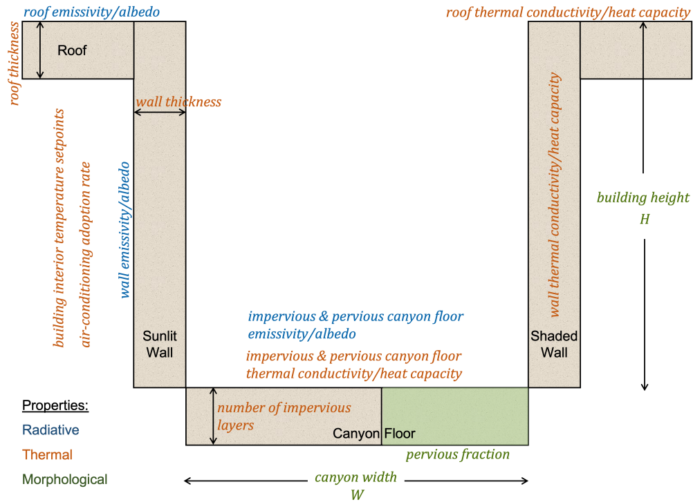
Figure 1. Conceptual schematic of an urban canyon to represent urban landscapes in CLMU (adapted from Oleson et al., 2008a). Properties are color-coded: blue for radiative, orange for thermal and green for morphological. Note that roof and wall thickness (despite being related to urban morphology) are considered thermal properties, as they are primarily used as weighting factors to calculate conduction fluxes into and out of canyon surfaces in CLMU (Lawrance et al., 2018; Oleson et al., 2010).
