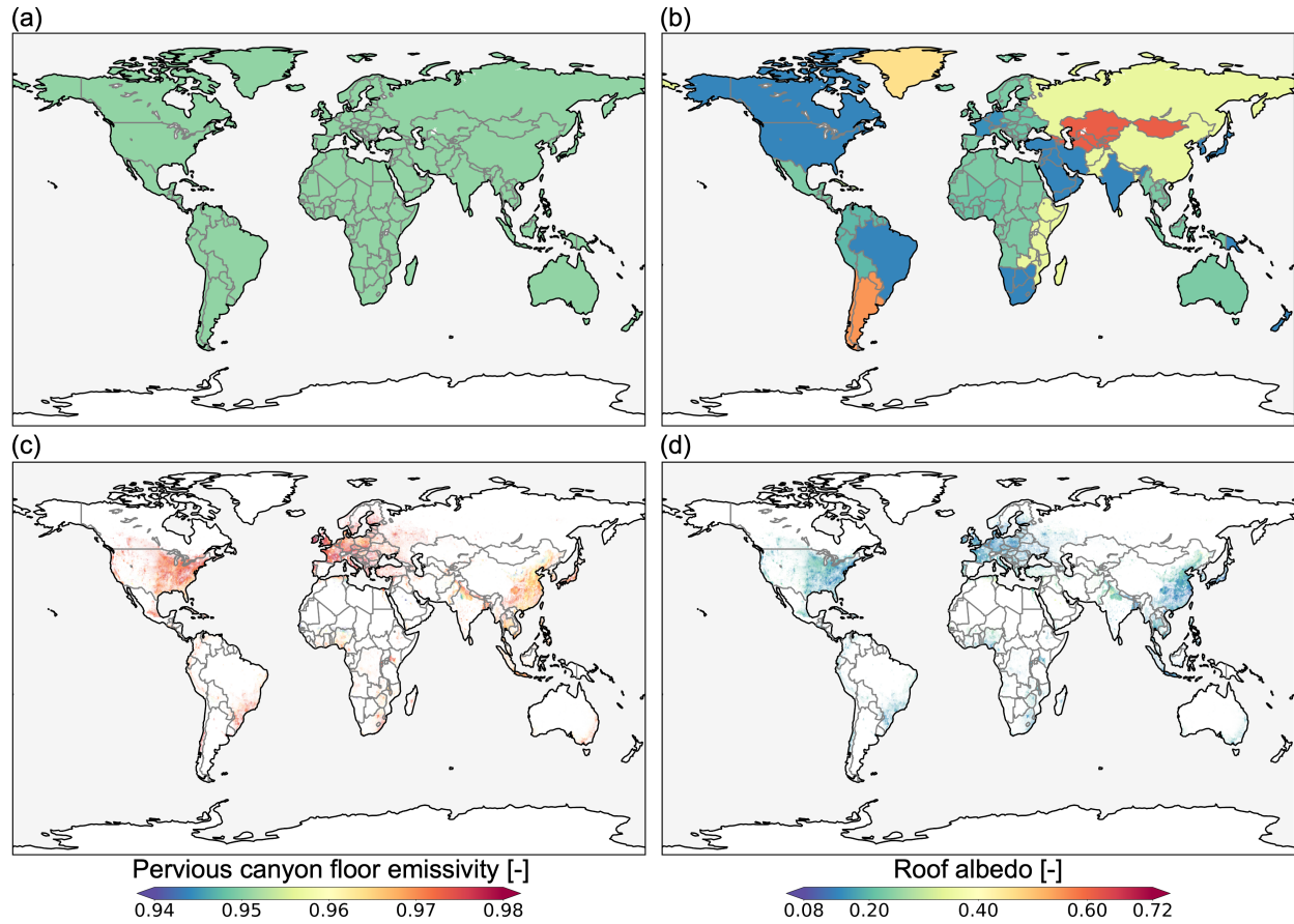
520 Figure 4. Global-scale comparison between the default CLMU and U-Surf parameters. (a, b) Discrete pervious canyon floor emissivity [unitless] and roof albedo [unitless] over 33 regions (area-weighted averages across TBD, HD and MD) in CLMU; (c, d) 1-km continuous pervious canyon floor emissivity and roof albedo in U-Surf. Each column shares the same color scale range but note that default CLMU parameters only have discrete values over 33 regions and 3 density classes.
