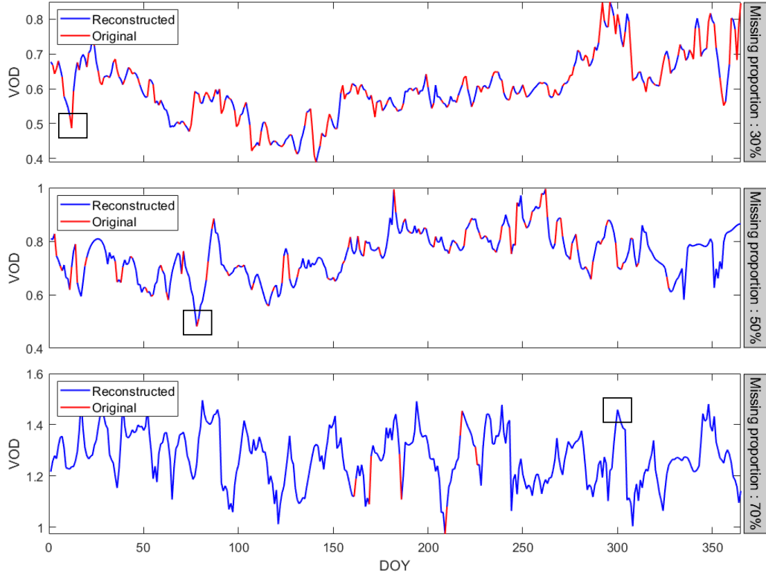
Fig. 6. Results of temporal variation in selected pixel at different missing data ratios in 2018, with magenta-red representing original values, blue representing model reconstructed values, and rectangles emphasizing some extreme value reconstruction results.
