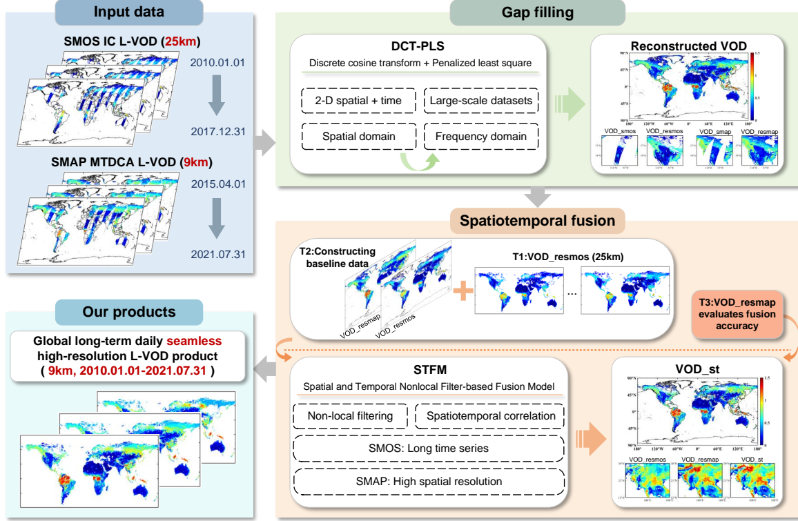
Fig. 3. General flow chart of the experiment.
