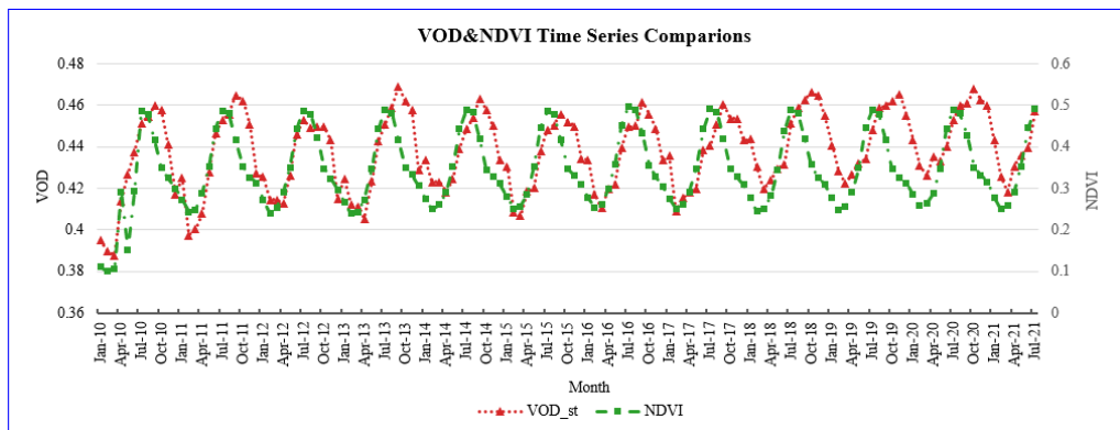
Fig. 21. Long - term monthly average trend comparison between VOD and NDVI.
