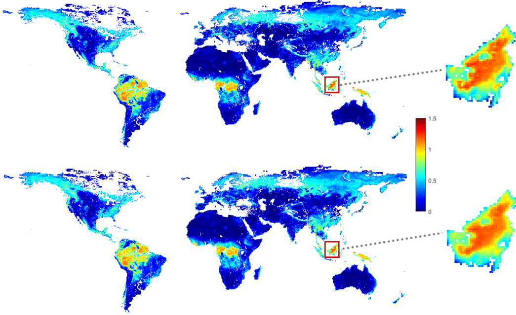
Fig. 19. Original (top) and reconstructed (bottom) results for July 2015 SMOS VOD monthly average. At a global scale, the overall coverage remains consistent. The red boxes highlight local areas, indicating that the monthly average spatial variations in the reconstructed data are smoother and free of striping.
