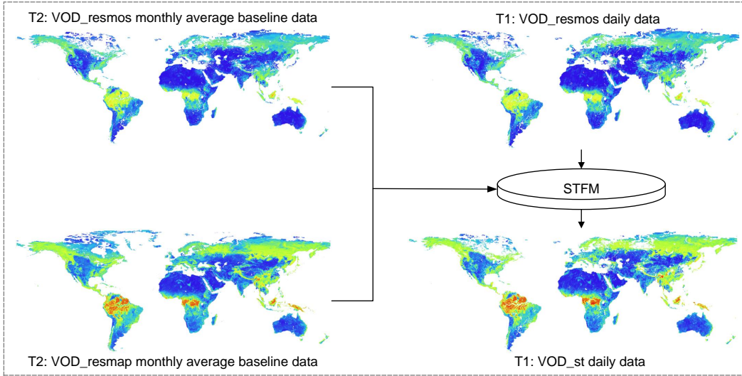
Fig. 2. Spatiotemporal fusion Process.
