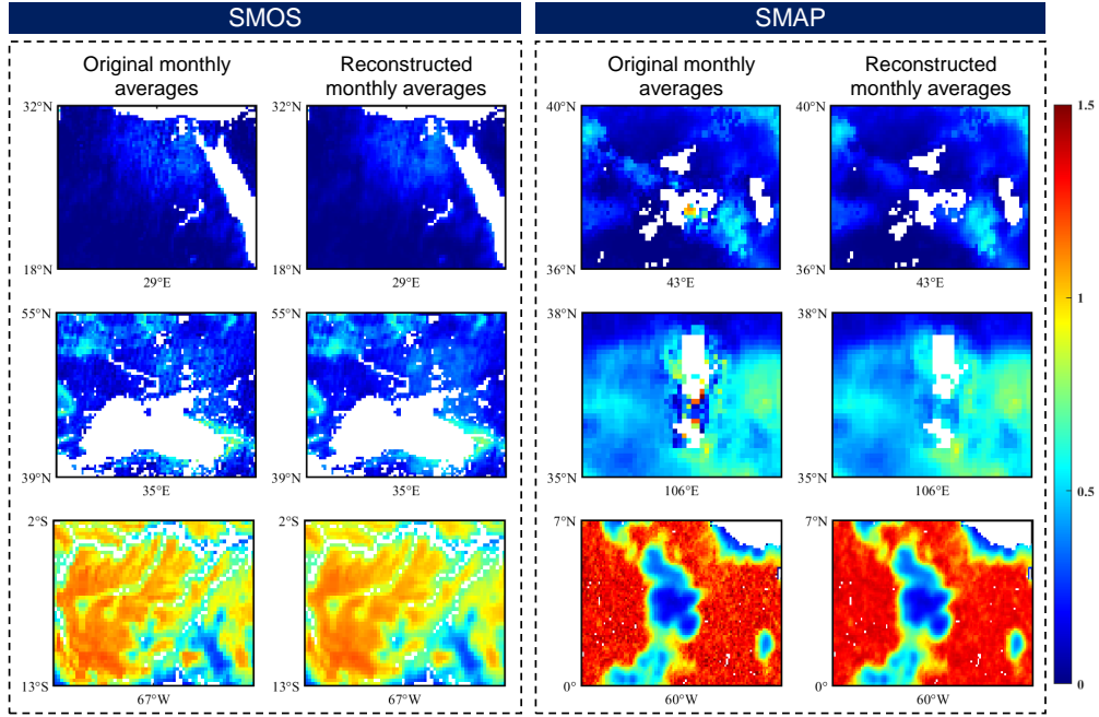
Fig. 20. Here three regions are selected for each type of satellite product to compare the monthly average results of original and reconstructed data under different factors.
