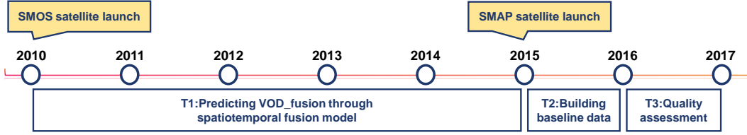
Fig. 1. Spatiotemporal fusion experiment time segment division explanation.
