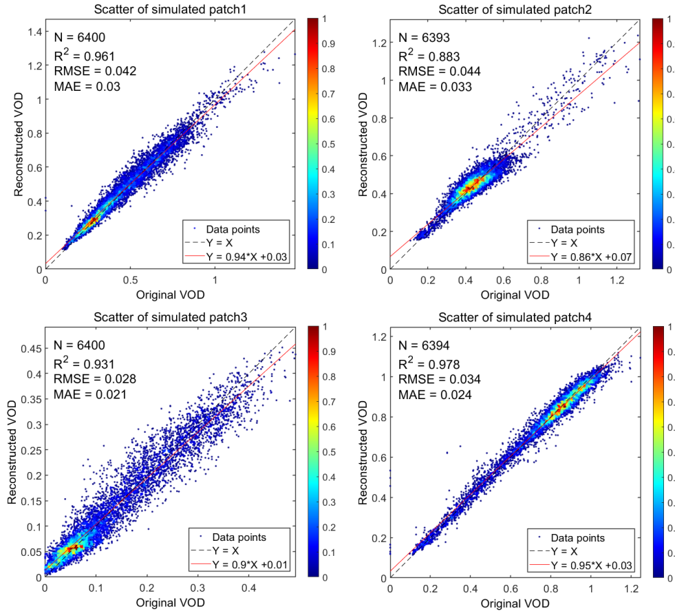
Fig. 10. Scatter plots of the original and reconstructed data for the four simulated missing regions on 20 July 2020. The colors and the color bar indicate the density of data points in the scatter plot.
