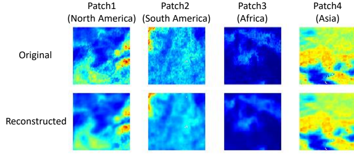
Fig. 9. Detailed original and reconstructed spatial information of four simulated missing patches. The four simulated missing patches ( 80 \times 80 pixel) are from the original SMAP L-VOD data from 20 July 2020, taken from North America, South America, Africa, and Asia.
