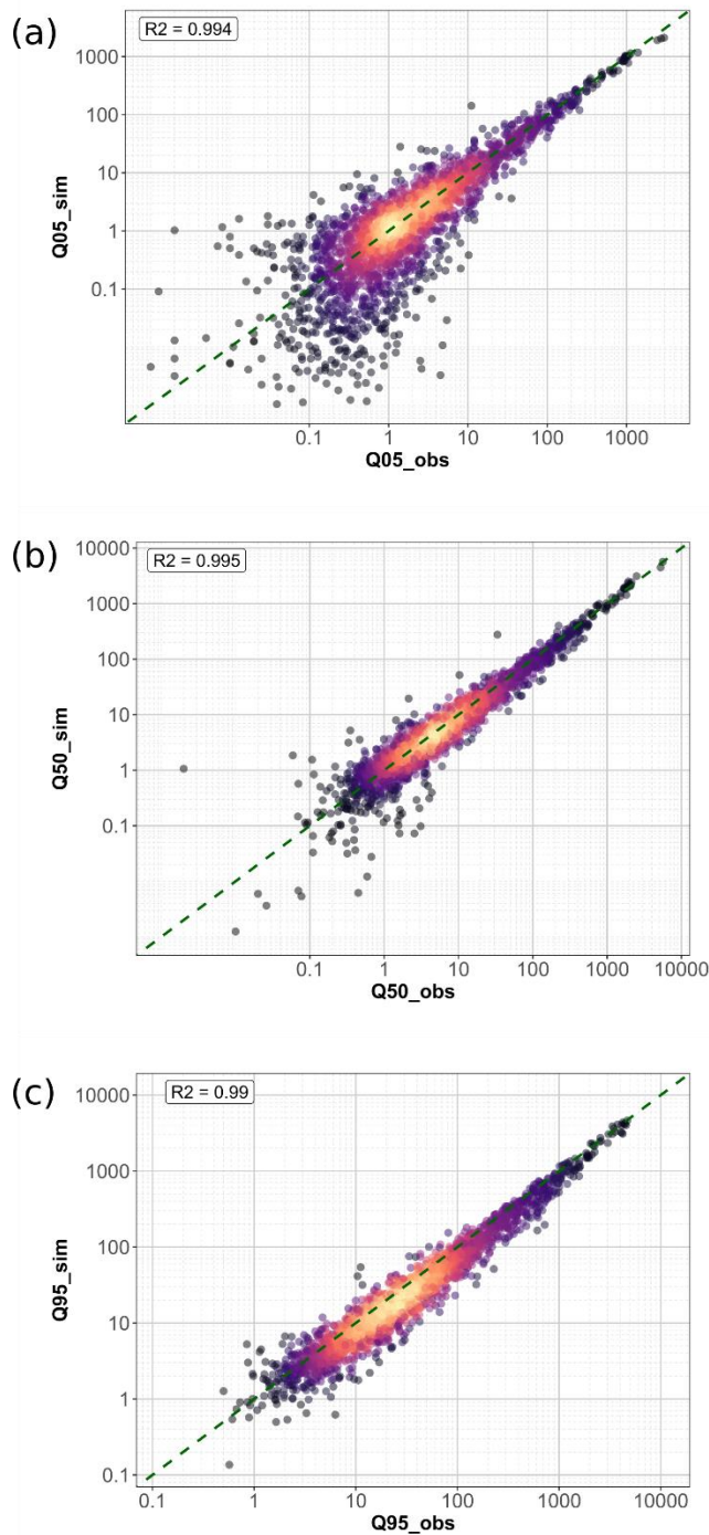
540 Figure 8: Scatterplot of observed versus simulated river flow quantiles [ \text{m}^3/\text{s} ]: (a) 5% quantile, (b) median (q50), (c) 95% quantile (q95) for the 2448 River gauges.
