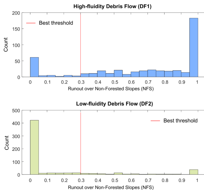
345 Fig. 8. Comparison of debris flows with high fluidity (upper) and low fluidity (lower) in the Casola Valsenio municipality, analyzed through the ratio of runout over non-forested slopes (NFS). The red line indicates the optimal threshold for distinguishing between the two types of landslides.
