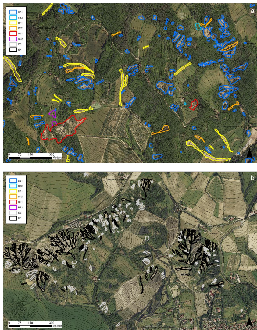
445 Fig. 13. Example images from the landslide inventory showing two representative area in coarse-grained units (a) and in fine-grained units (b).
