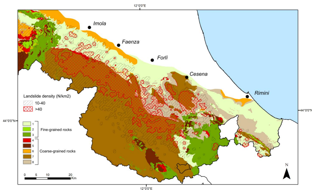
380 Fig. 10 Detail of the Romagna area showing two classes of landslide density (between 10 and 40 landslide/km 2 and more than 40 landslide/km 2 ) with the eight lithological units in background.
