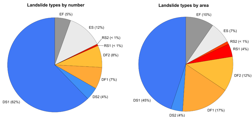
Fig. 11. Pie charts showing the percentage of landslide types by number (left) and by area (right).
