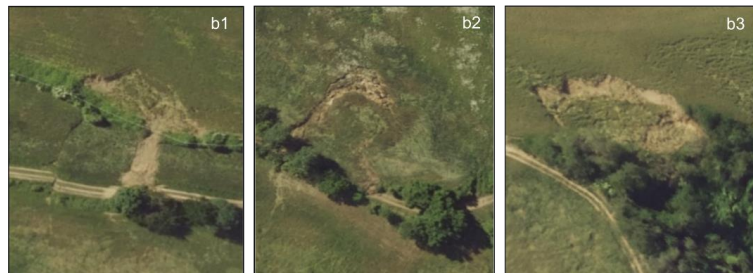
Fig. 3. Representative images of the two distinct types of debris slides caused by the May 2023 event.
