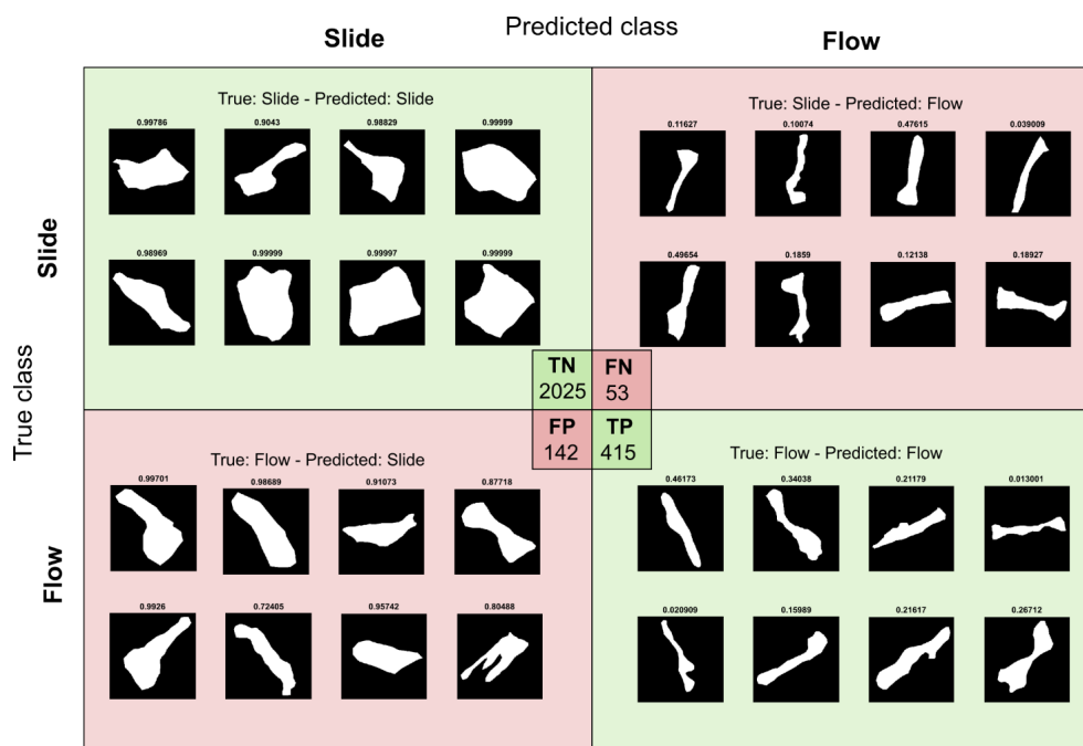
Fig. 6. Outcomes from the Convolutional Neural Network model applied to differentiate slides from flows using the shape of the polygons. The figure displays the confusion matrix for the testing dataset, which includes 50% of the landslides manually mapped in the Casola Valsenio municipality; TN=True Negative; FN=False Negative; FP=False Positive; TP=True Positive. The small polygons in each category represent example landslides that are correctly (TP, TN) or incorrectly (FP, FN) classified.
