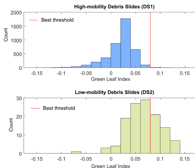
305 Fig. 7. Comparison of the frequency distributions of the Green Leaf Index for high-mobility debris slides (upper) and low-mobility debris slides (lower) manually mapped in Casola Valsenio municipality. The red line marks the optimal threshold distinguishing the two landslide types.
