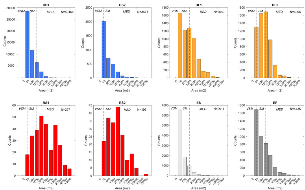
Fig. 12. Frequency histograms depicting size of various landslide types. The classes labeled at the top of each chart (VSM=very small; SM=small; MED=medium) correspond to the size classification proposed by McColl and Cook (2024).
