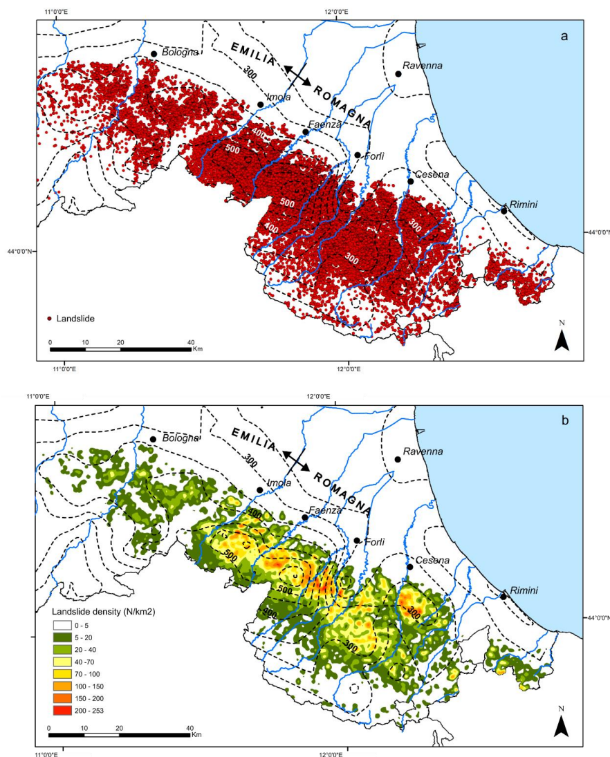
Fig. 9. a) Map showing the distribution of the 80997 landslides triggered by the May 2023 event in the Emilia-Romagna region, manually mapped and represented as individual points. b) Density map calculated as the number of landslides per 1 km 2 cell.
