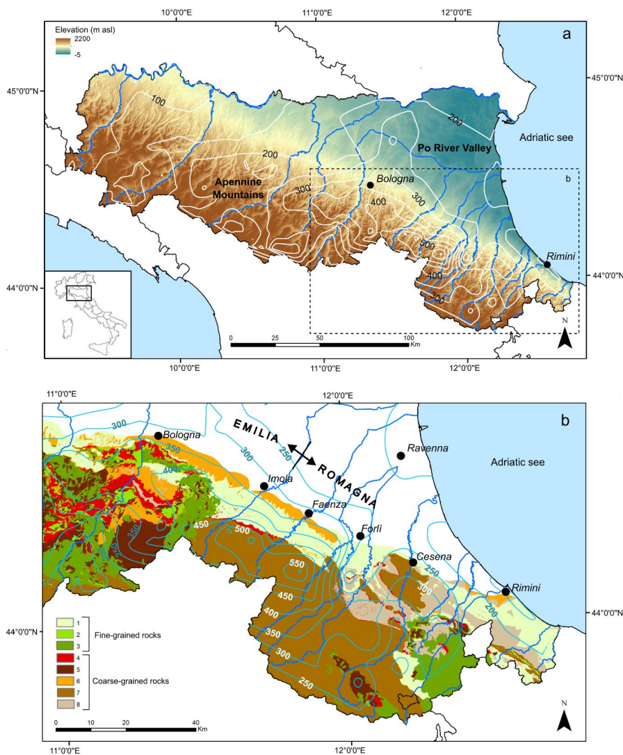
Fig. 1. a) Overview map of the Emilia-Romagna region (Italy), illustrating elevation and cumulative rainfall isohyets from May 1-17, 2023. b) Detailed view of the area most impacted by the event, featuring the geological units referenced in Table 1.
