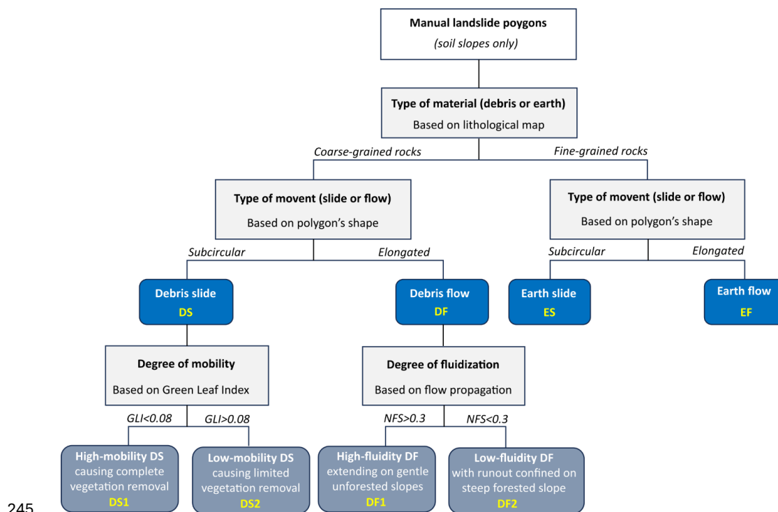
Fig. 5. Flowchart depicting the process used to ensure data quality and standardize the classification of manually mapped landslides.
