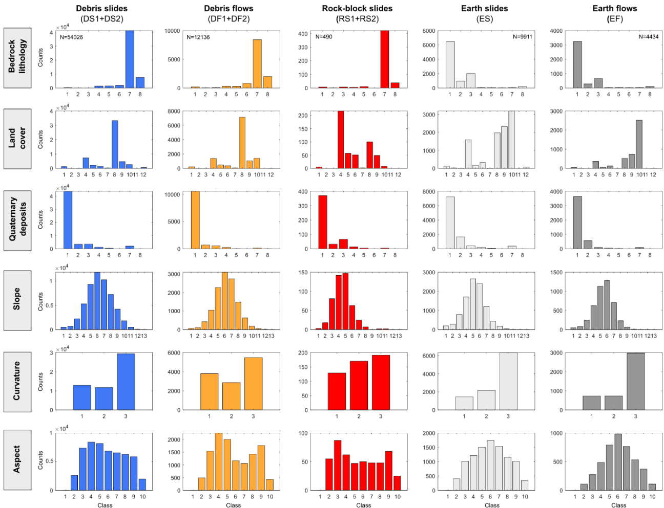
Fig. S1. Frequency histograms for the six spatial variables detailed in Table S1, across different types of landslides. Each histogram represents the number of landslides whose source area—defined by a 10-meter radius circle at the upper part of the polygon—falls within specific factor classes
