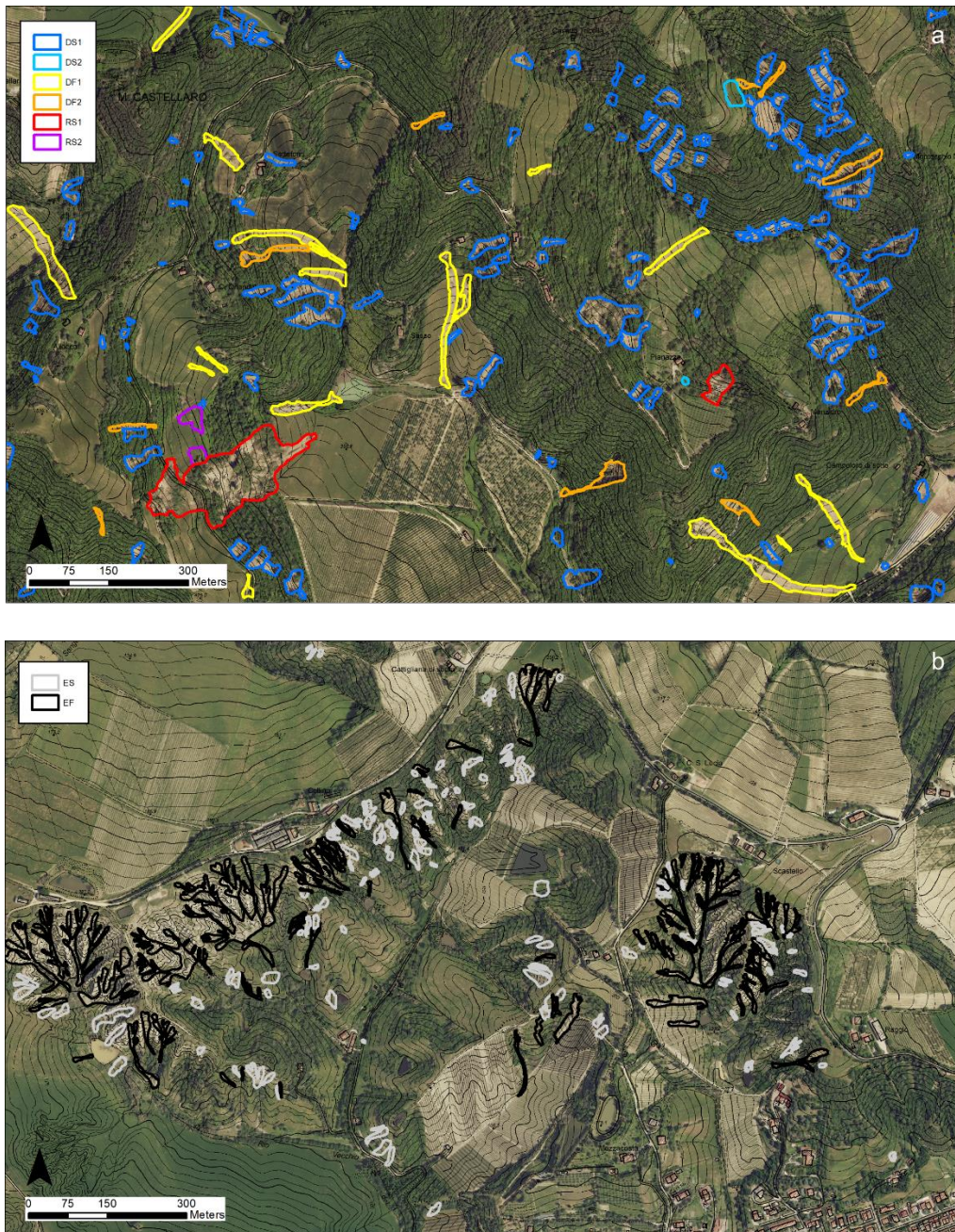
485 Fig. 15. Example images from the landslide inventory showing two representative area in coarse-grained units (a) and in fine-grained units (b). DS1=debris slide with high mobility; DS2=debris slide with low mobility; DF1=debris flow with high fluidity; DF2=debris flow with low fluidity; RS1=fully-developed rock-block slide; RS2=incipient rock-block slide; ES=earth slide; EF=earth flow.
