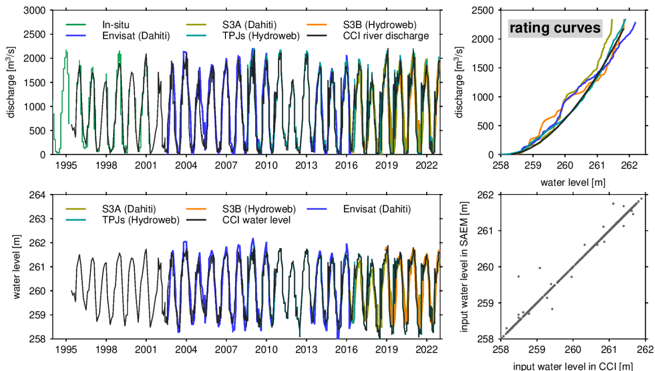
Figure 10. Comparison of discharge and water level time series between SAEM and the CCI project for the Niger River. (Top-left) Discharge time series from SAEM’s four mission series and CCI, alongside in-situ measurements. (Top-right) Rating curves were derived from each time series using non-parametric (SAEM) and parametric (CCI) approaches. (Bottom-left) Water level time series from SAEM and CCI. (Bottom-right) Scatter plot showing the correlation between water levels in SAEM and CCI data sets. The consistency across data sets highlights the reliability of satellite-derived measurements for river discharge estimation.
