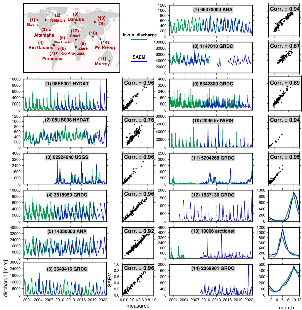
Figure 7. Comparison of estimated discharge from the SAEM data set with in-situ discharge measurements across selected gauges from various continents and data centers. For cases 1 to 11, where simultaneous data were available, the time series plots are shown alongside scatter plots and their corresponding correlation coefficients (displayed to the right of each time series plot). For cases without simultaneous data between SAEM and gauged discharge (cases 12, 13, and 14), the monthly means are compared. It should be noted that in the scatter plots, the values are normalized by the maximum discharge value among the simultaneous gauge and SAEM data sets.
