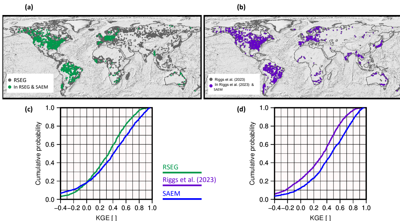
Figure 9. Comparison of the developed SAEM data set with two existing data sets: RSEG and the data set from Riggs et al. (2023). (a) Spatial distribution of the gauges in RSEG in grey and the gauges common with SAEM in green. (b) Same as (a) but between SAEM and Riggs et al. (2023). (c) CDF of the KGE values for the common gauges between SAEM and RSEG with simultaneous in-situ data. (d) Same as (c) but between SAEM and Riggs et al. (2023).
