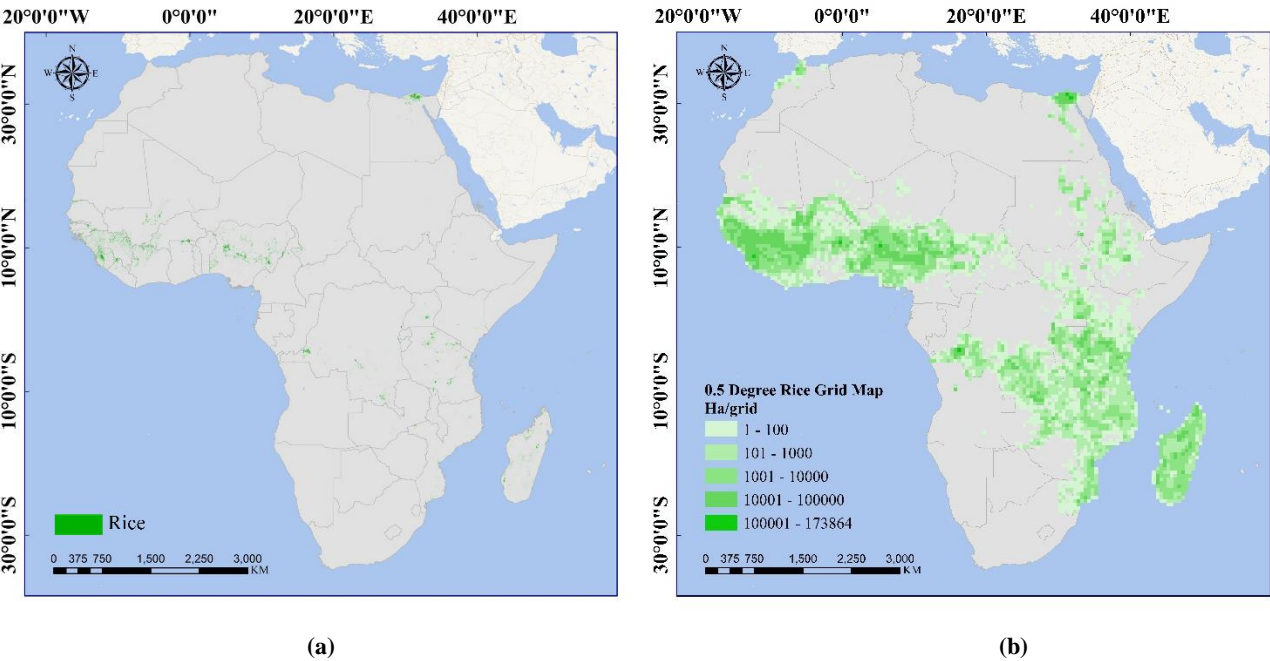
325 Figure 10. Rice mapping result in Africa (a) 20-meter spatial distribution map (b) corresponding 0.5° grid map
