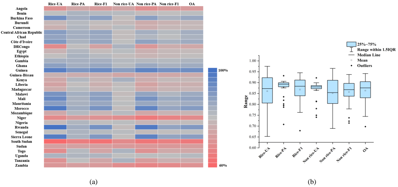
Figure 13. Performance on validation set (a) heat map of validation accuracy across 34 African countries (b) corresponding box plot
