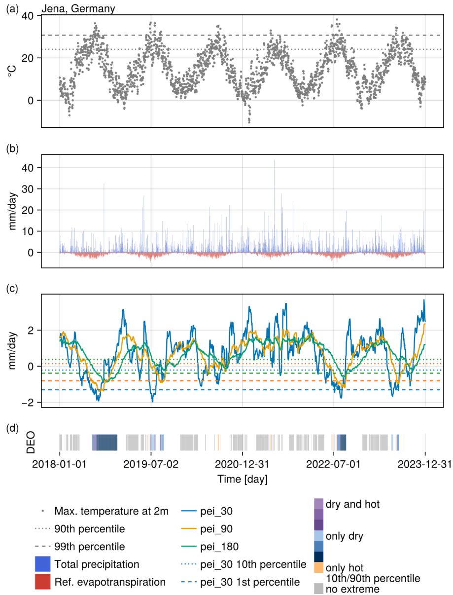
Figure C1. Timeseries (2018–2022) of (a) maximum daily temperature, (b) daily precipitation and reference evapotranspiration, (c) the three drought indicators (PEI) and (d) the Discrete Extreme Occurrences (DEO) around the city of Jena, Germany. The summers in those years (except 2021) were relatively dry, with very hot days resulting in compound dry and hot extremes in 2018, 2019 and 2022.
