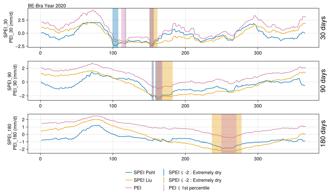
Figure D1. Time series of daily PEI 30 , PEI 90 , and PEI 180 (PEI) and daily SPEI from two independent datasets (Pohl: EOBS based, (Pohl et al., 2023); Liu: ERA5 based, Liu et al. (2024)) at one ICOS site in Belgium for the year 2020. The vertical lines show the days detected as extremely dry.
