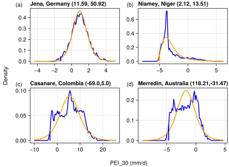
Figure A3. Probability density functions of PEI 30 values at four locations: in blue the empirical distribution, in orange the fitted distribution. The vertical lines show the 1 % threshold and the shaded area under the curve the probability of extremes.
