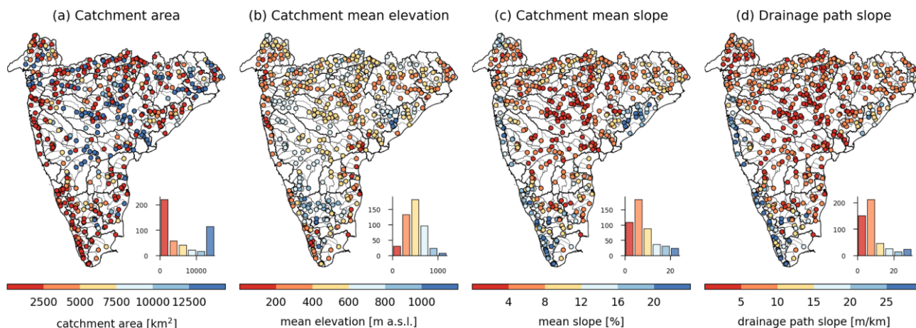
Figure 3. Topographic characteristics of catchments in Peninsular India. The histograms depict the frequency distribution of catchments across the bins. (a) catchment area in km 2 , (b) catchment mean elevation in meters above mean sea level, (c) catchment mean slope in percentage, and (d) catchment mean drainage path slope in m/km.
