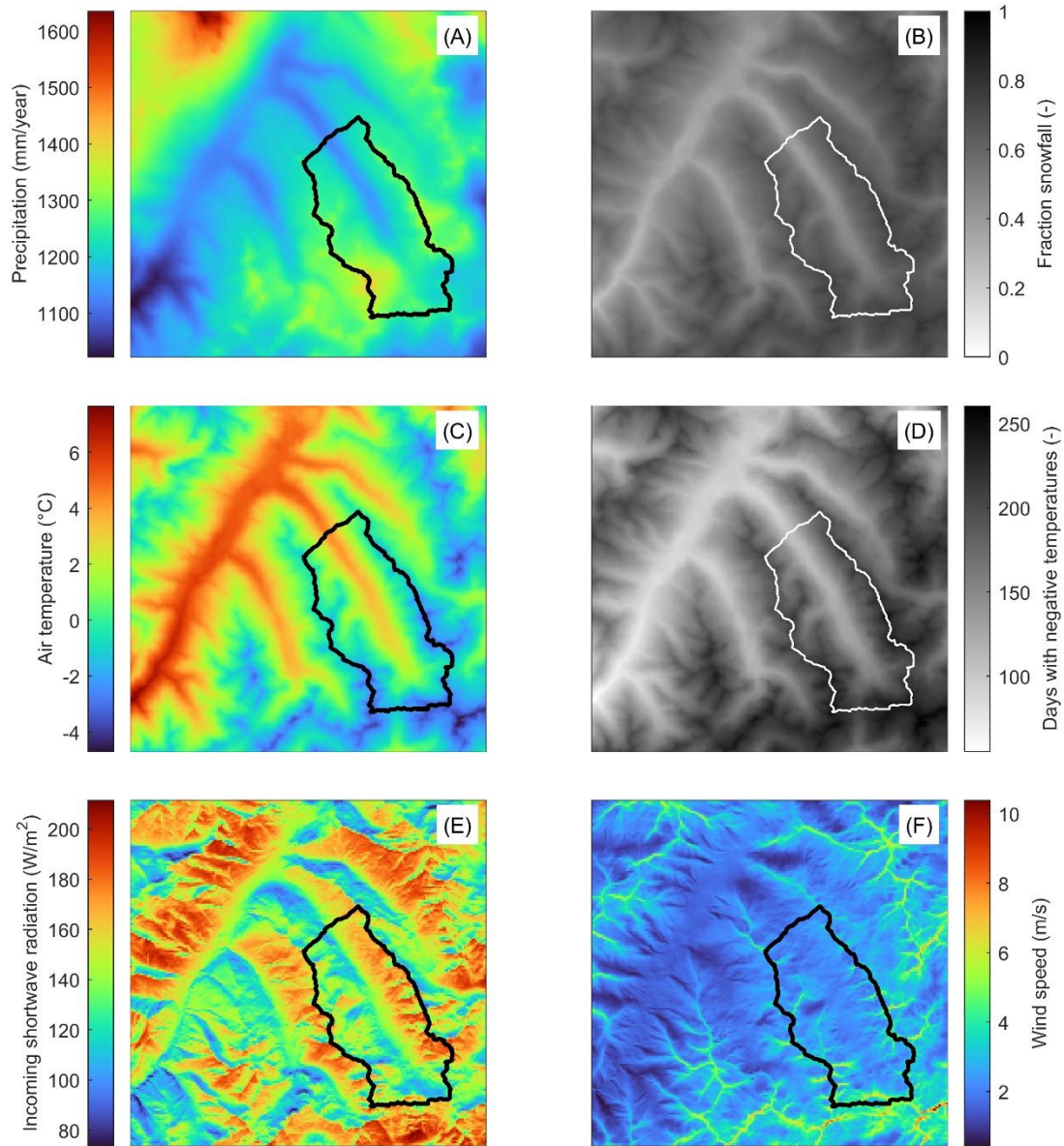
Figure 2. Panel a shows the average annual precipitation over the study period, while panel b illustrates the fraction of total precipitation that falls as snow. Panel c presents the mean air temperature during the study period, and panel d displays the fraction of days with a daily average air temperature below zero degrees Celsius. Finally, panel e depicts the mean incoming shortwave radiation, and panel f visualises the average wind speed over the data period.
