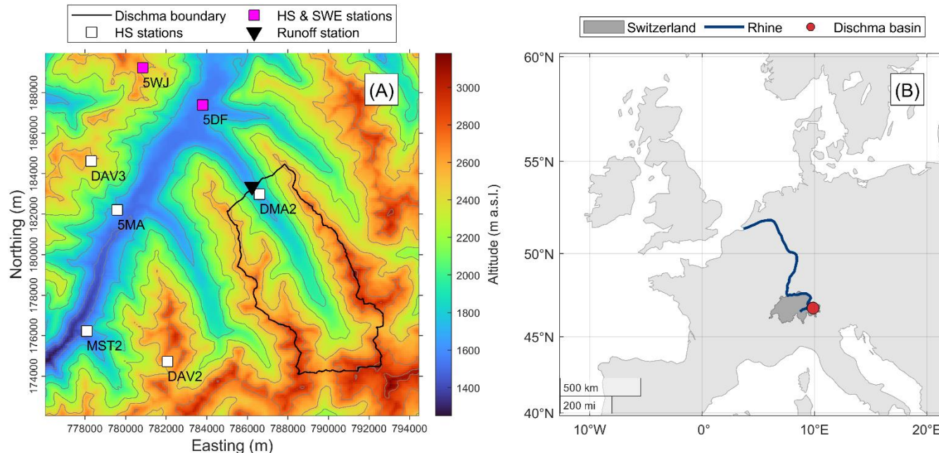
Figure 1. Site map of the Dischma watershed and extended domain for which we provide meteorological and land cover data (panel a). The map indicates the altitude of the domain as well as the location of stations used for snow, meteorological and runoff measurements. Location of the Dischma basin in Europe along with the Swiss national borders and the Rhine river (panel b).
