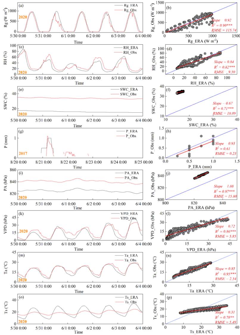
Fig.1 Comparison ERA5-land variables vs observation
