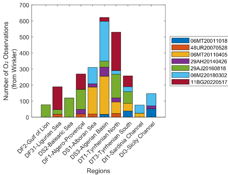
Figure 4. Reference cruises: (a) Map showing the location of reference stations; (b) vertical distribution of dissolved oxygen data from Winkler measurements, including the mean profile across all reference cruises; and (c) number of reference oxygen observations (Winkler measurements) per region.
