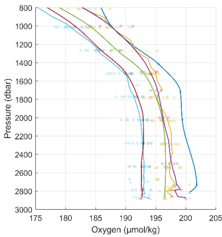
Figure 7. Average vertical profiles of dissolved oxygen in (a) the Algerian basin (region DS3) and (b) the Tyrrhenian Sea (region DT1). Panels (c) and (d) provide a zoomed view of the deep layers below 800 dbar. Colored dots represent discrete Winkler oxygen measurements, color-coded by cruise, while the solid-colored lines indicate cruise-specific mean profiles.
