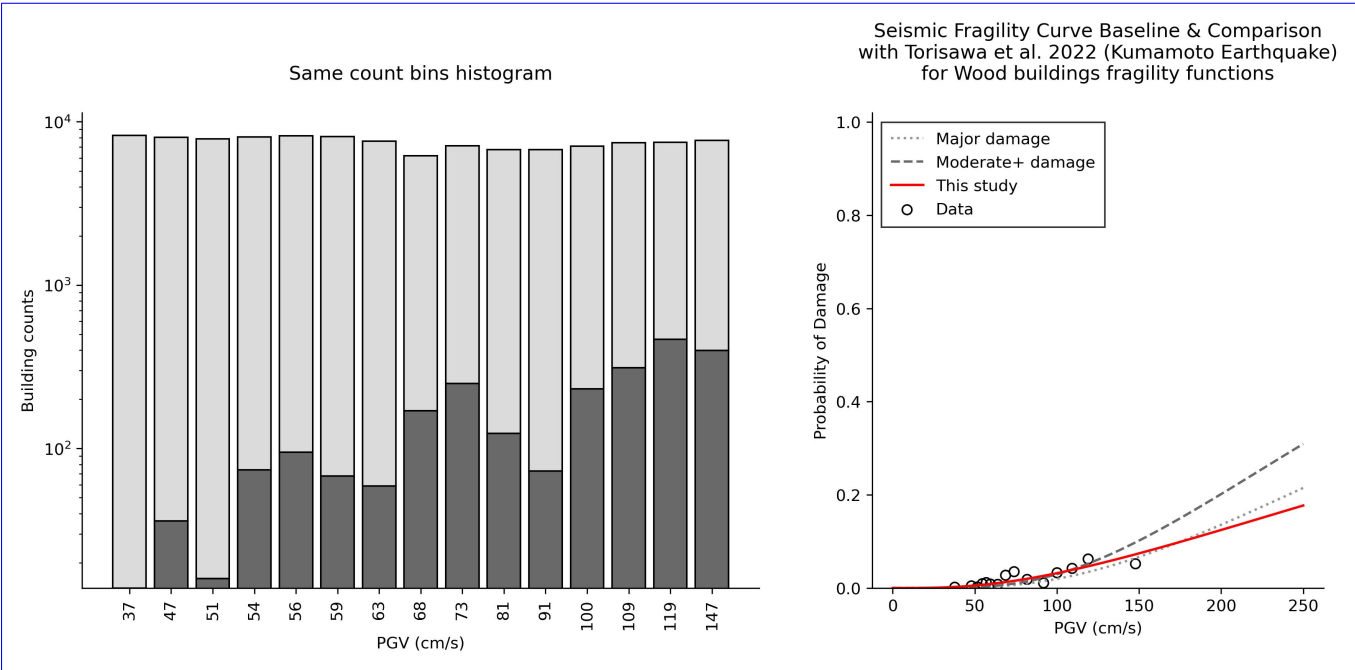
Figure 12. Left: Histogram of aggregated building damage. Right: Empirical fragility function (red solid line) for earthquake-affected buildings relative to PGV. We provide two wood buildings fragility functions for “Major” and “Moderate+” damage classes (respectively dotted line and dashed line) proposed by Torisawa et al. (2022) for buildings built between 2001 and 2016 and affected by the 2016 Kumamoto Earthquake.
