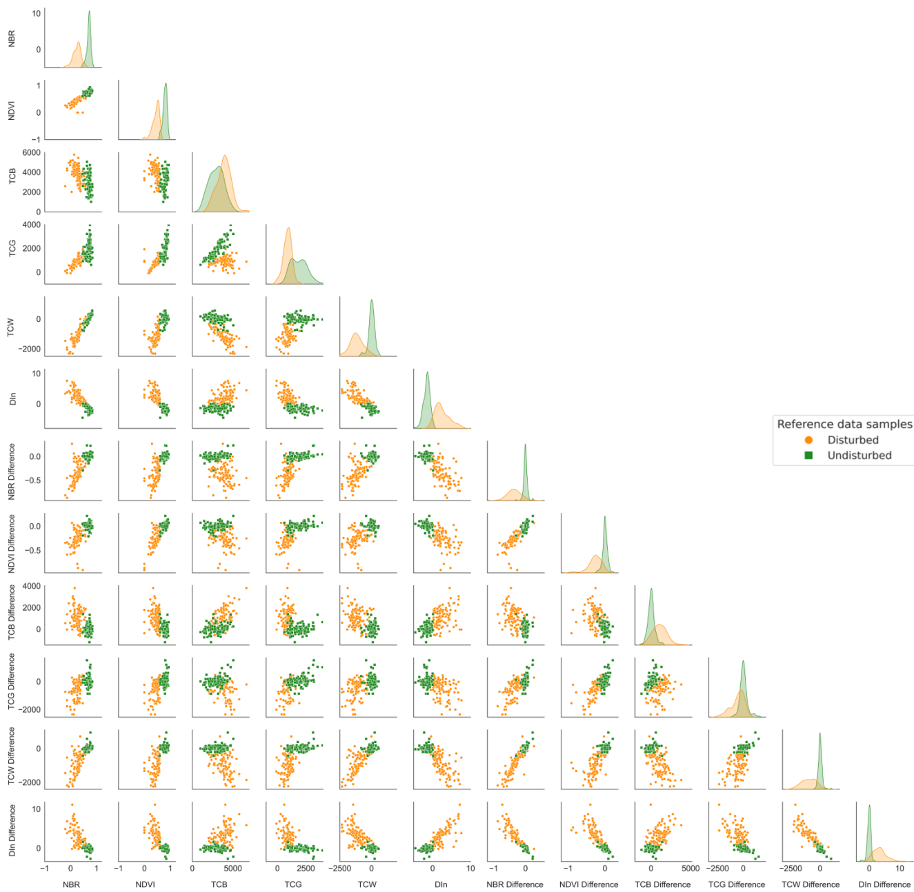
595 Figure A5. Feature space of spectral indices for disturbed and undisturbed reference samples.
