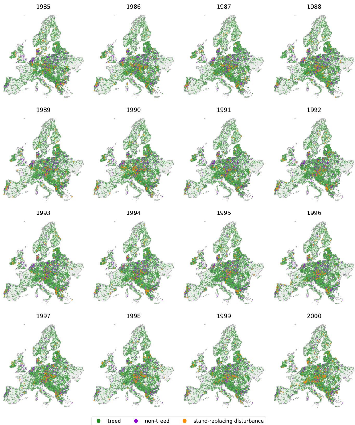
Figure A3. Maps of annual reference data within forests for disturbance and undisturbed (treed and non-treed). Continue in A3(b).
