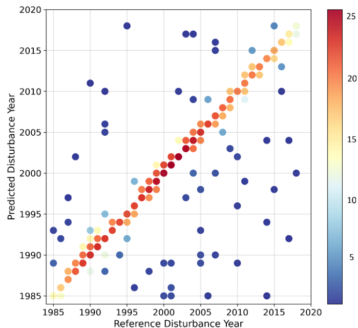
375 Figure 9. Validation of the disturbance year. Estimated disturbance year versus manually interpreted year of disturbance for independent reference pixels (colour bar indicates the number of points)
