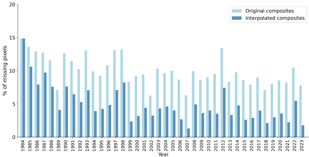
Figure A2. Annual percentage of no-data pixels for best available pixel composites and after linear gap-filling interpolation.
