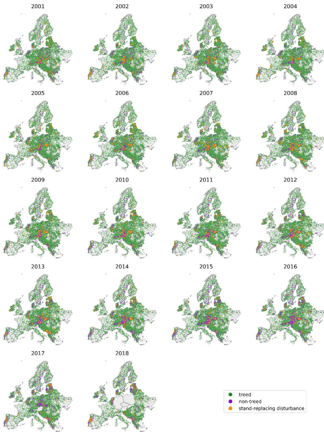
585 Figure A3. Maps of annual reference data within forests for disturbance and undisturbed (treed and non-treed). Continuation from A3(a).
