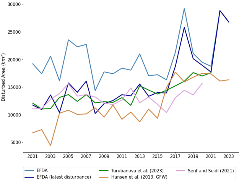
Figure 10. Annual disturbed area estimates from current available datasets for Europe.
