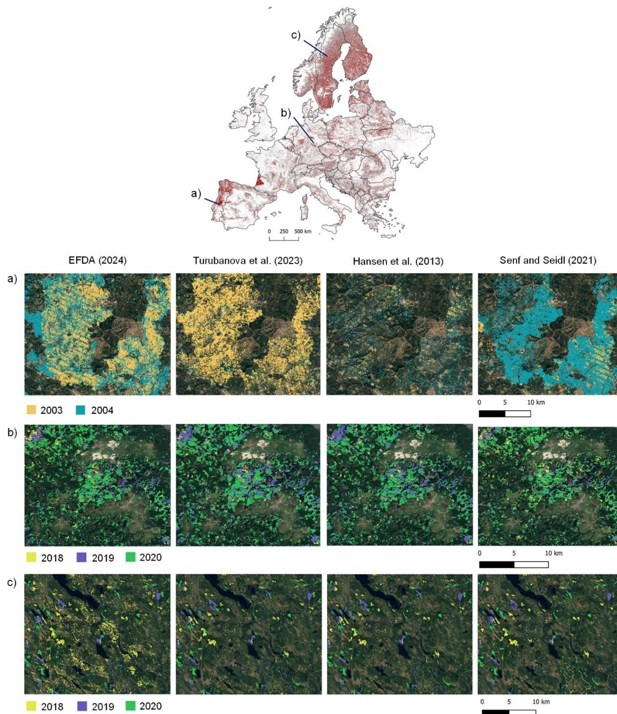
470 Figure 11. Examples of disturbance maps from different datasets for (a) fires in Central Portugal, (b) bark beetle outbreaks in Central Germany, (c) harvests in northern Sweden.
