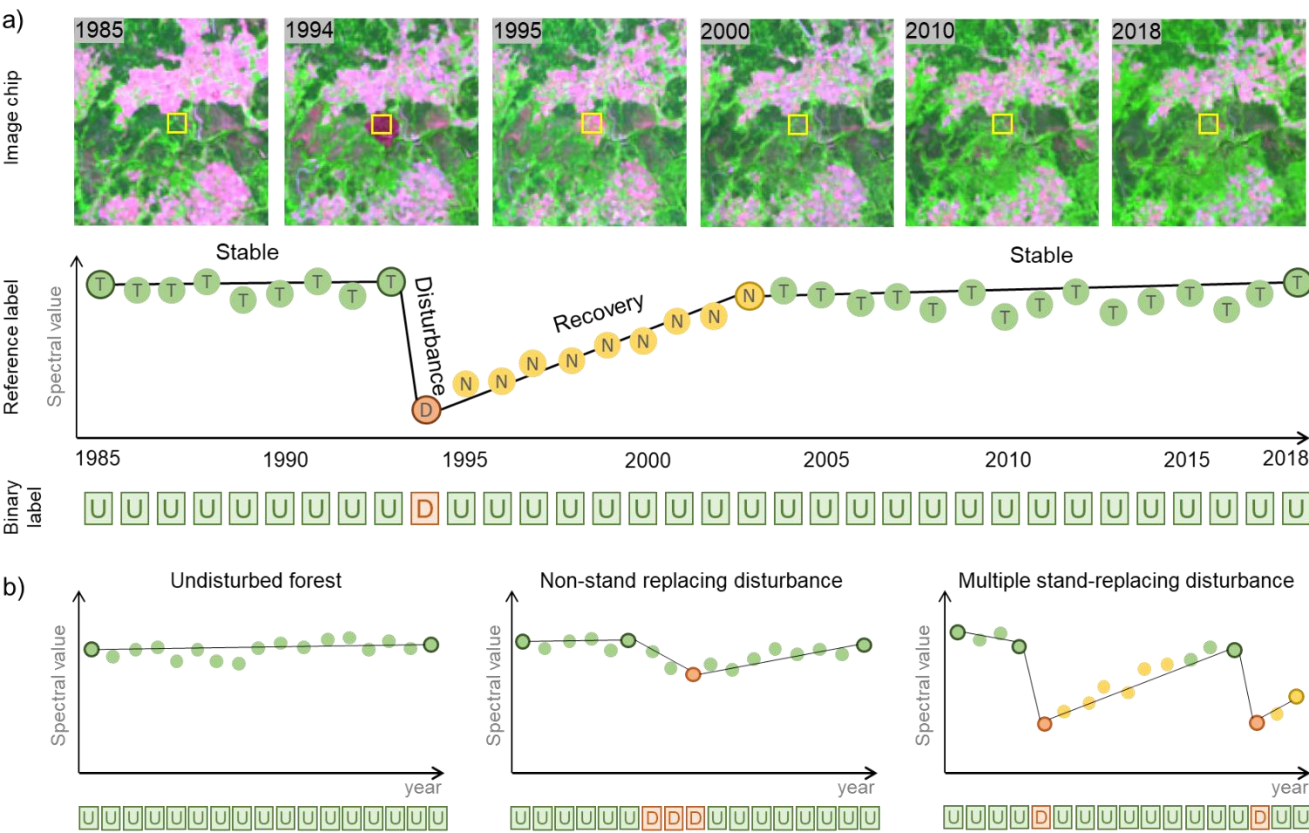
170 Figure 3. Schematic representation of the original reference data from Senf et al. 2018 and Senf et al. 2021: a) Image chips and corresponding segmentation labels of stable forest, disturbance and recovery segments and corresponding land cover of treed (T) and non-treed (N), ultimately labelled into annual binary classes of Undisturbed (U) and Disturbed (D); b) examples of undisturbed forest, a gradual non-stand replacing disturbance and multiple stand-replacing disturbances, and their corresponding binary labels.
