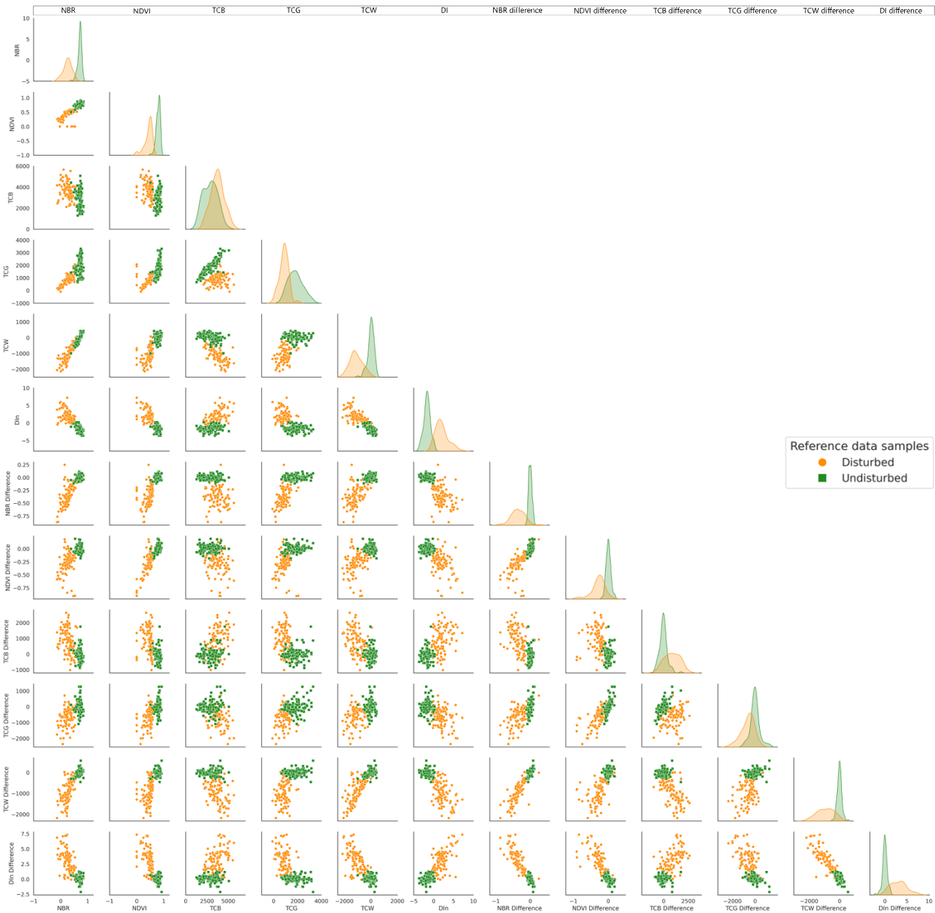
Figure A5. Feature space of spectral indices for disturbed and undisturbed reference samples.
