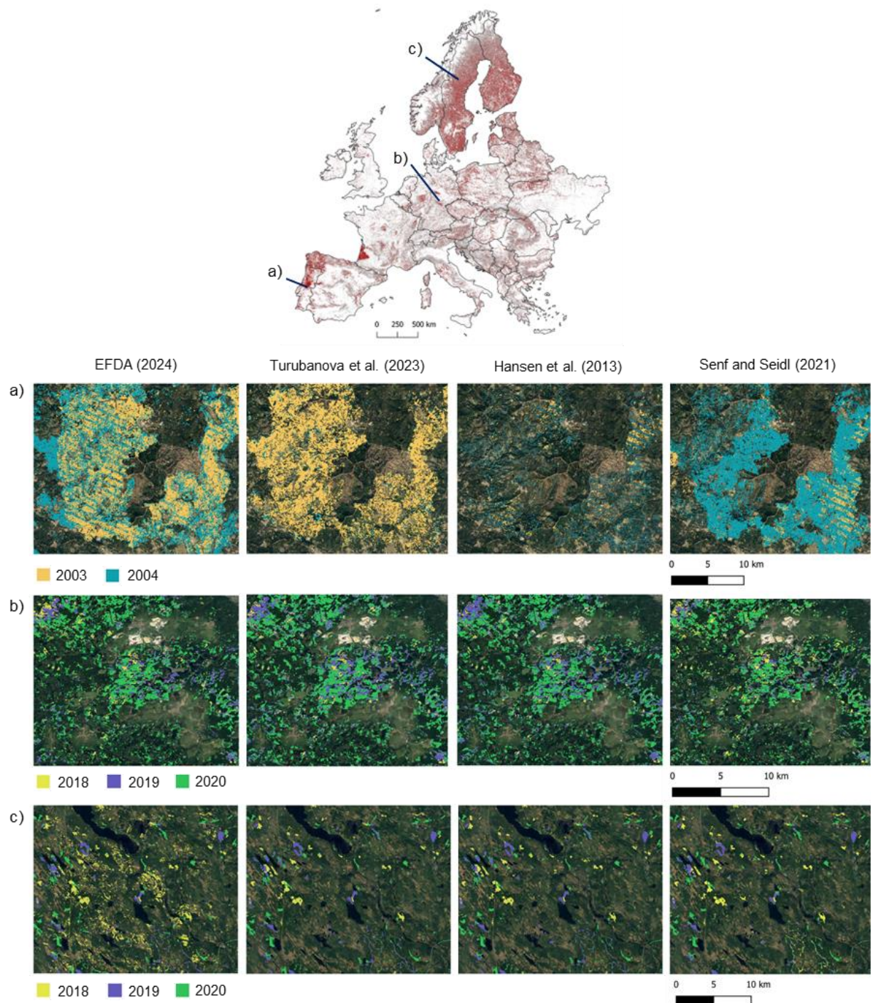
Figure 11. Examples of disturbance maps from different datasets for (a) fires in Central Portugal, (b) bark beetle outbreaks in Central Germany, (c) harvests in northern Sweden.
