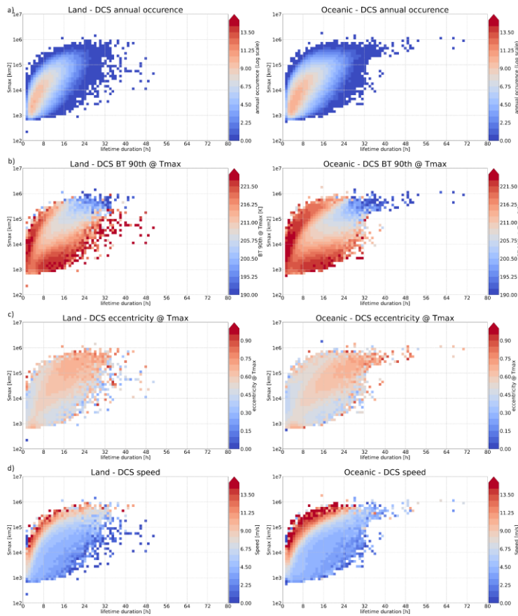
500 Figure 9 (a) annual occurrence of the deep convective systems for continental (left) and the oceanic region; (b) 90 th percentile
