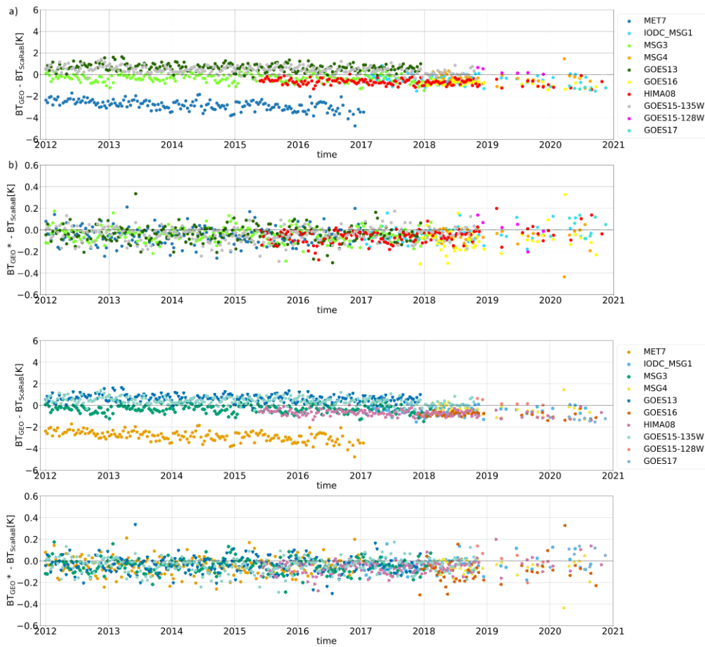
Figure 1 (a) Time series of initial BT bias of geostationary IR observations with respect to SCARAB in the range [180 K- 205 240 K] between 2012 and 2020; (b) after spectral and calibration corrections.
