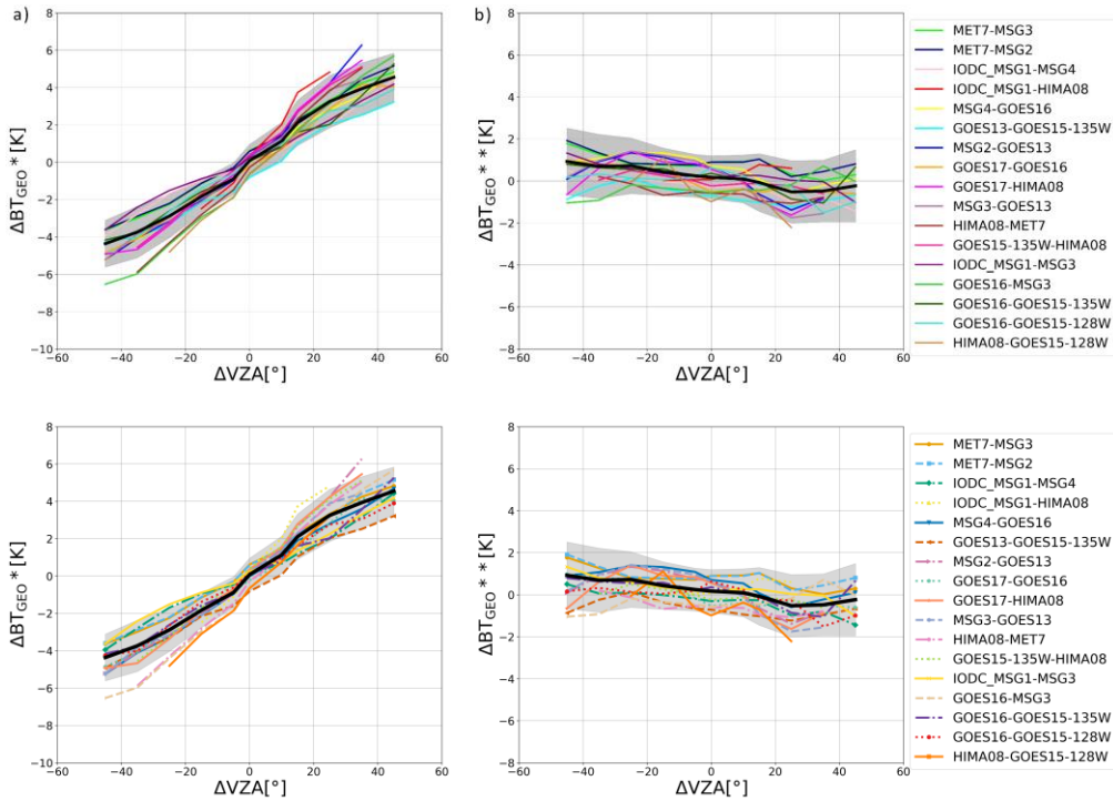
Figure 2 (a) Variation of the BT bias according to the VZA differences between pairs of geostationary platforms observing common areas and for BT_{SCARAB} in the range [180 K-235 K] between 2012 and 2020 before Viewing Zenith Angle corrections; (b) after Viewing Zenith Angle corrections. The BT bias and its standard deviation for all the pairs of geostationary platforms are represented respectively by the black line and the filled area in grey.
