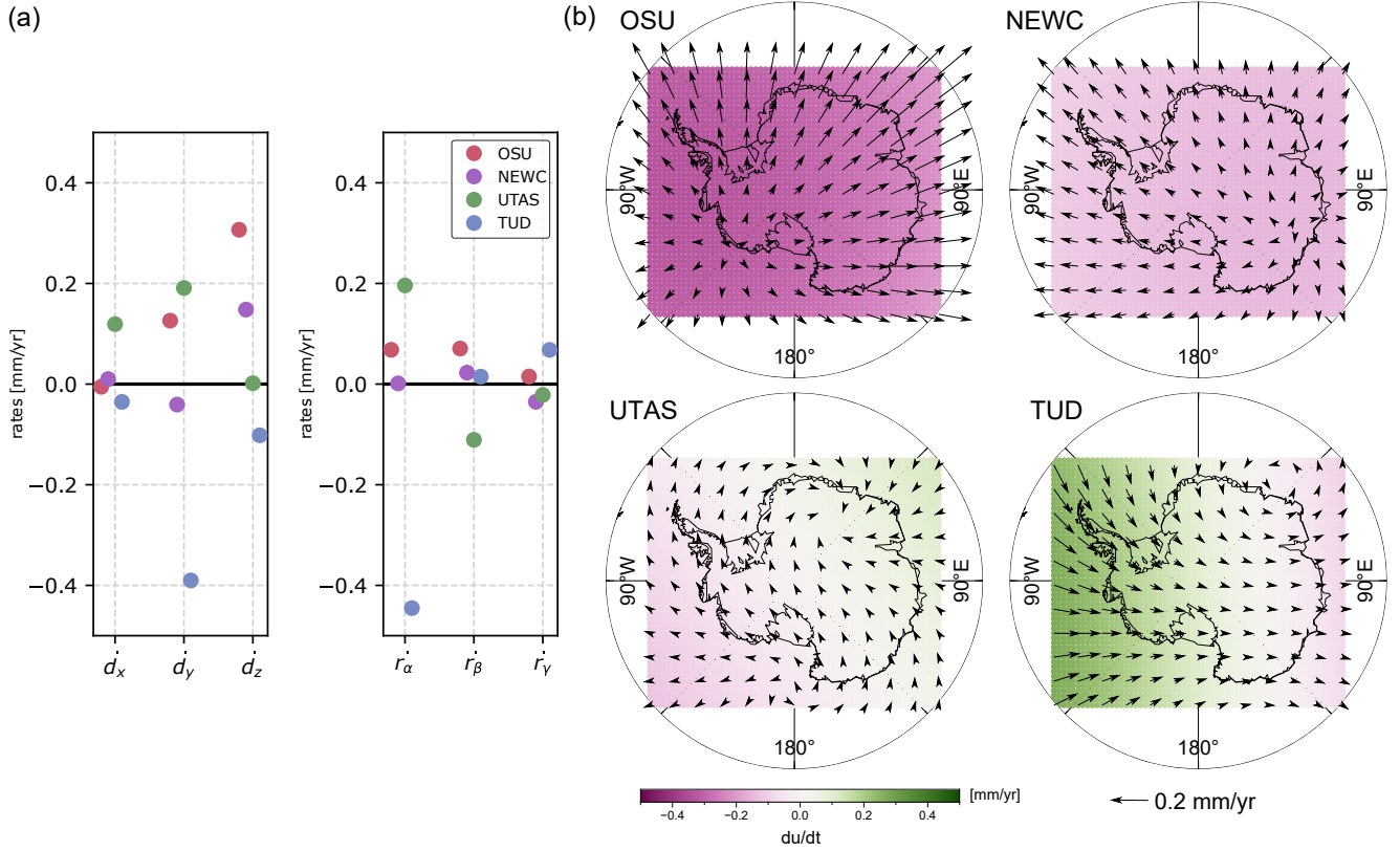
Figure 3. (a) Linear rates of translation and rotation the six Helmert Parameters for AC solutions w. r. t. IGB14 based on a selection of regionally distributed IGS sites. Angular velocities \dot{\alpha}_j , \dot{\beta}_j , \dot{\gamma}_j are multiplied by the Earth radius to obtain tangential velocities r'_\alpha , r'_\beta and r'_\gamma for better comparability to translation parameters. A positive angle describes a clockwise rotation. The formal uncertainties are negligible, with a range of one to two magnitudes smaller than the estimated values. Panel (b) displays the applied linear rates of HP-HPs HP-HPs on a defined grid covering the study area. The coloured grid displays the local uplift rates, arrows the show lateral velocities.
