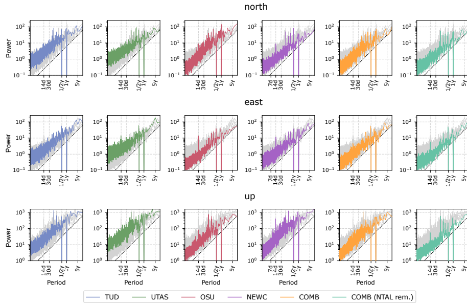
Figure 7. Median Lomb-Scargle periodograms of residual time series (east, north, up) for a selection of 29 cGPS sites for the four ACs and the combined solution with and without NTAL removed . Each LSP-plot displays the LSP of a specific solution in color and the LSPs of the other solutions in grey. The dashed line displays flicker noise with an arbitrary amplitude.
