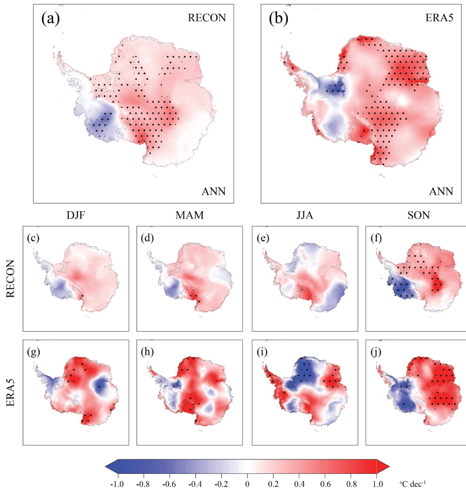
Figure 2: Annual linear temperature trends from RECON (a) and ERA5 (b) for 1998-2022; seasonal results for RECON (c-f) and ERA5 (g-j) are presented below these. The dots indicate statistical significance of the linear trends at the 0.01 level after considering the lag-1 autocorrelation after Santer et al. (2000).
